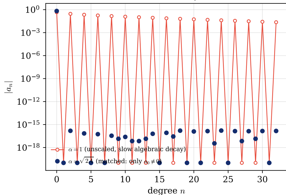
(b) Coefficient decay at A=8
