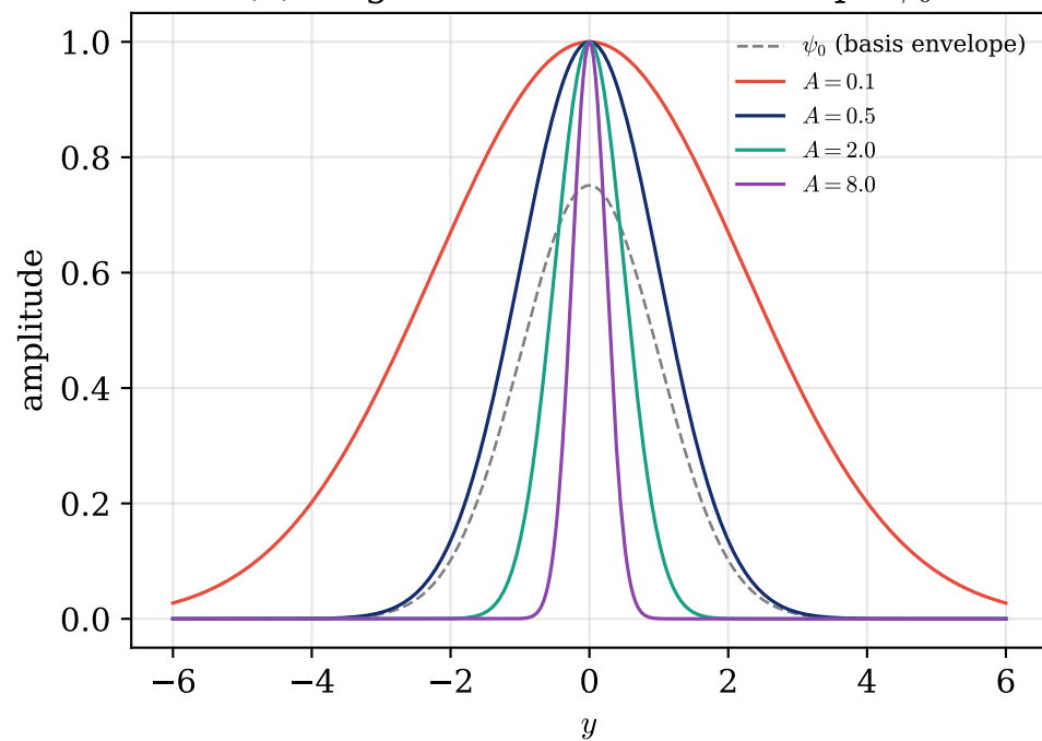
(a) target e^{-Ay^2} vs basis envelope \psi_0
