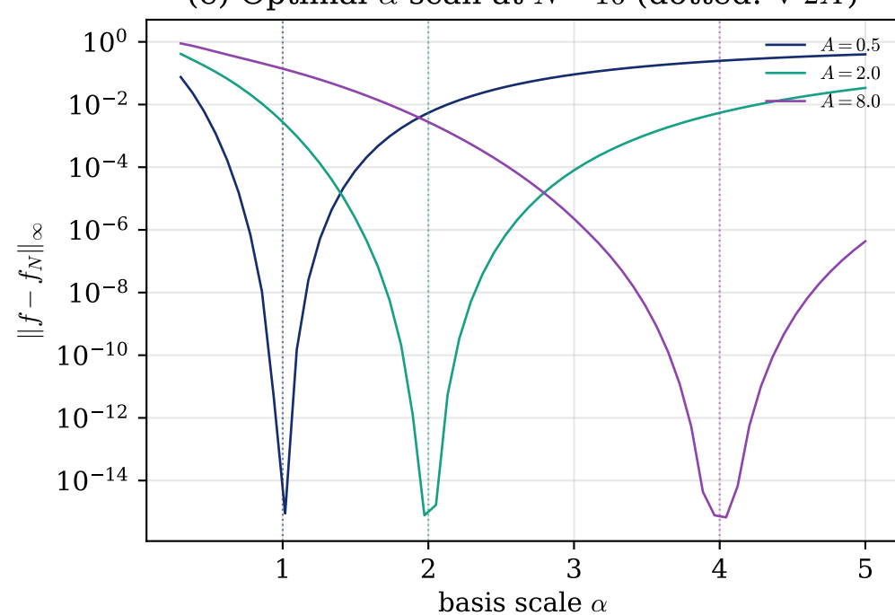
(e) Optimal- \alpha scan at N=16 (dotted: \sqrt{2A} )
