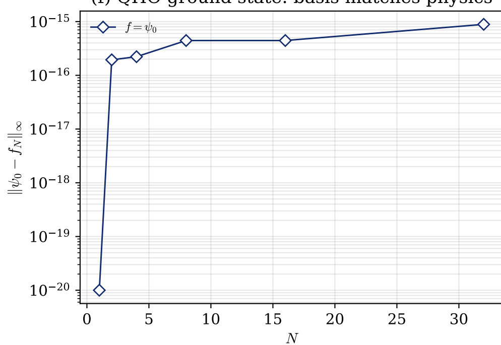
(f) QHO ground state: basis matches physics
