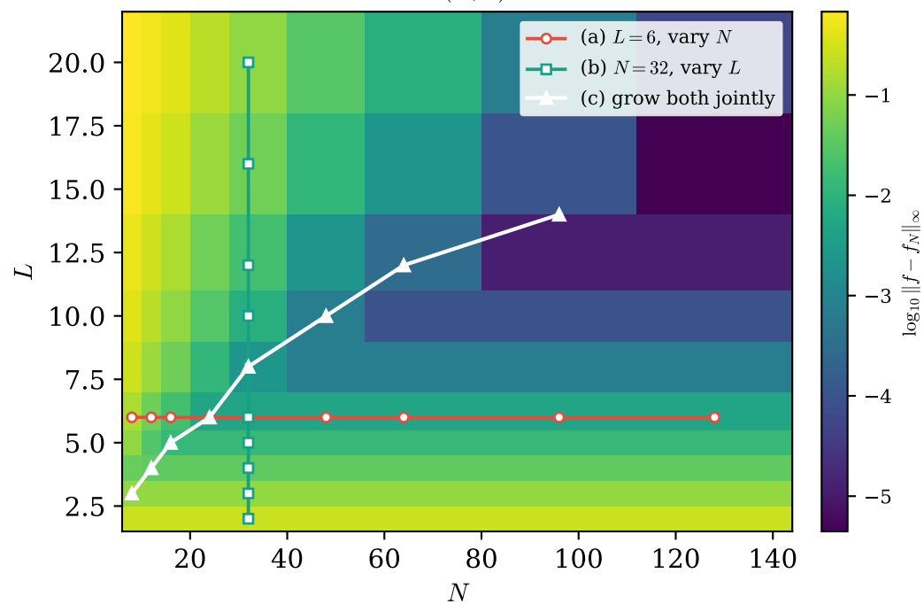
(d) the error surface E(N, L) and its three slices
