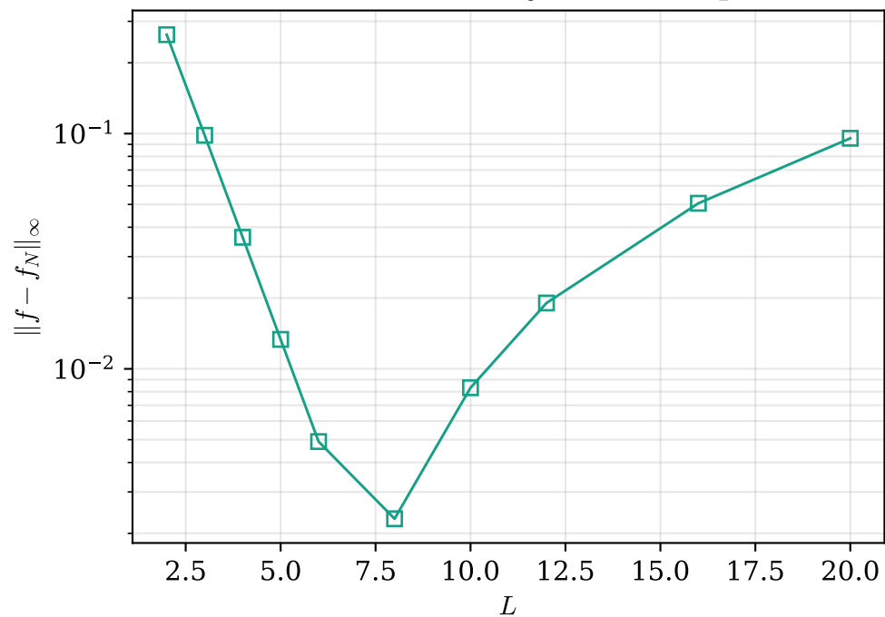
(b) Fix N=32 , vary L : sweet spot
