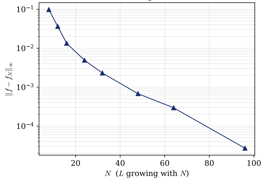
(c) Grow both: subgeometric descent
