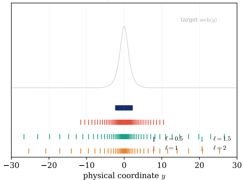
(b) \sinh -mapped grids at N = 64 for several \ell
