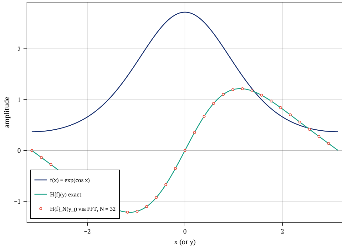
f(x) = \exp(\cos x) and its Hilbert transform on the circle
