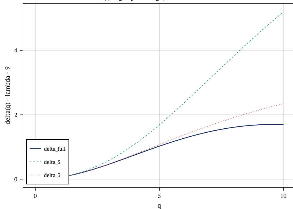
(f) ce_3: q/n^2 large, sideband breaks
