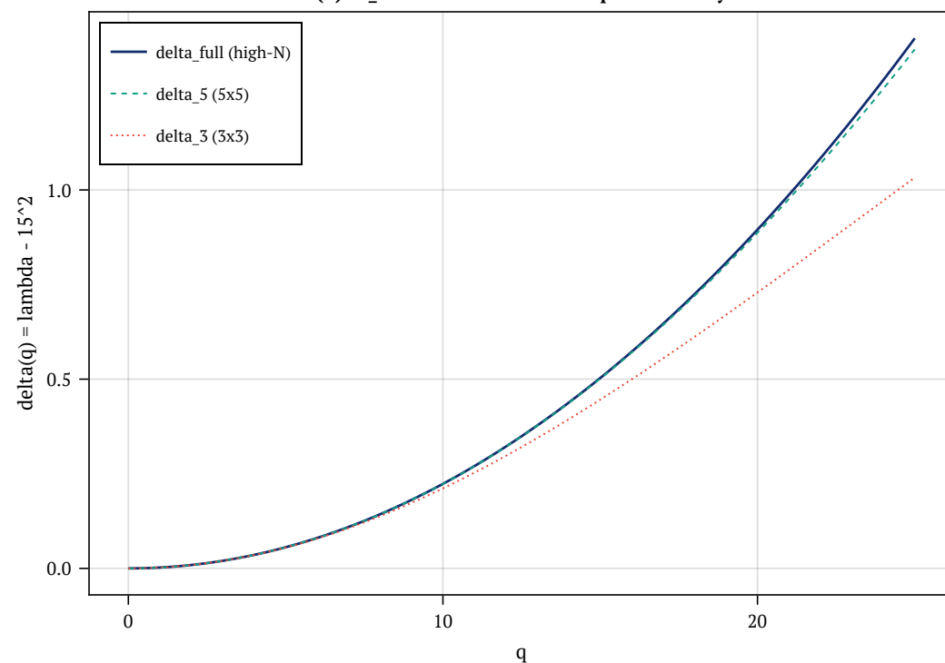
(d) ce_15: 5x5 matches full to plot accuracy
