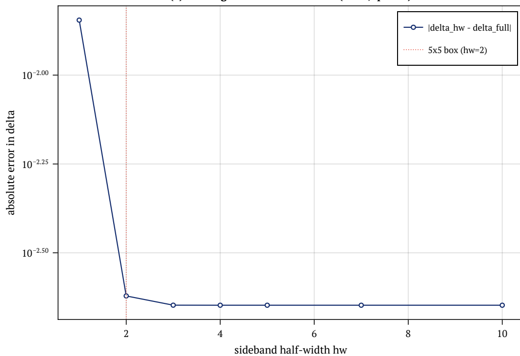
(e) convergence vs sideband size ( n=15, q=10.0 )
