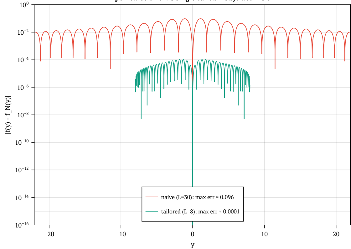
pointwise error: a single tuned L buys decimals
