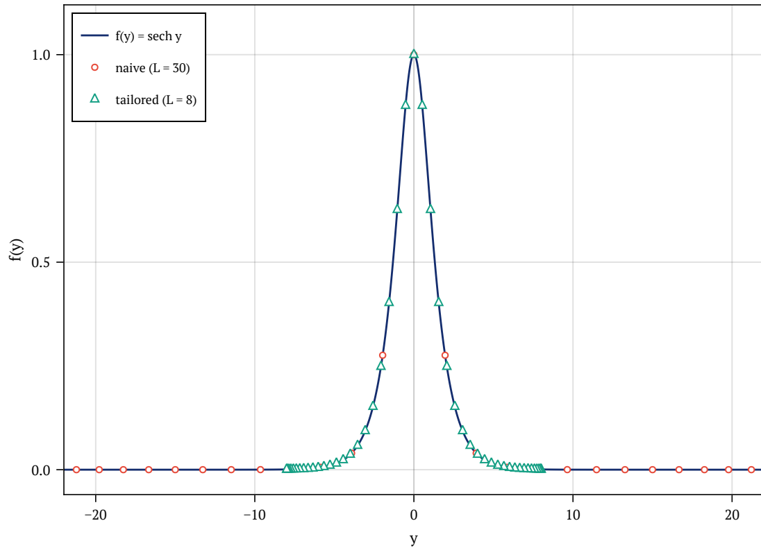
same f , same N = 48 , two truncation lengths L
