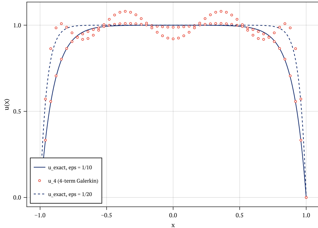
\epsilon^2 u'' - u = -1, u(\pm 1) = 0 : 4-term Galerkin vs exact
