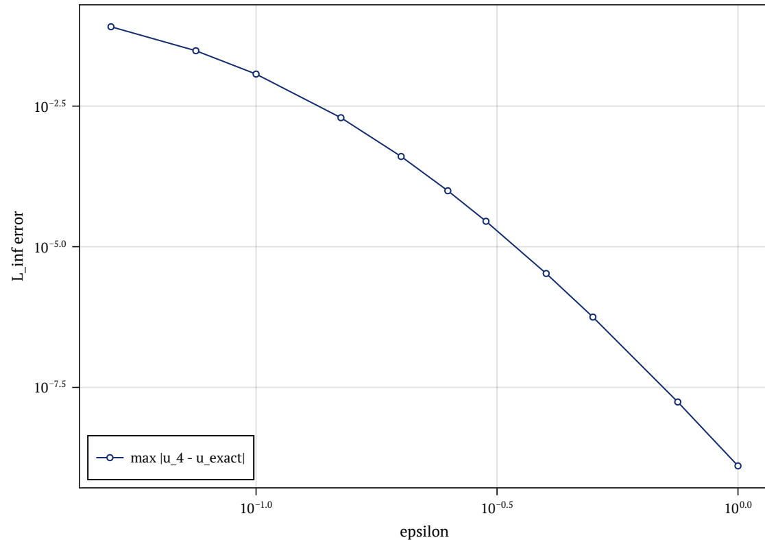
Boyd Table 20.3: 4-term symbolic accuracy across epsilon
