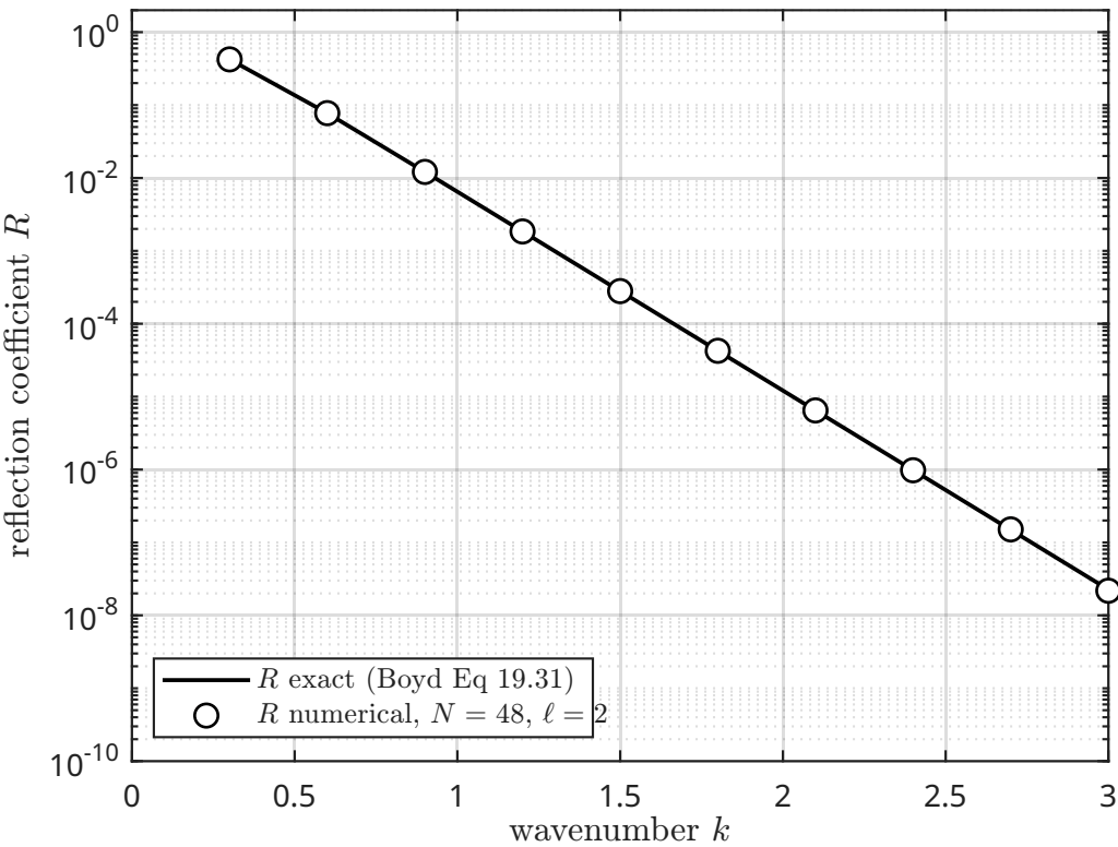
\text{sech}^2 scattering: spectral R matches the closed form
