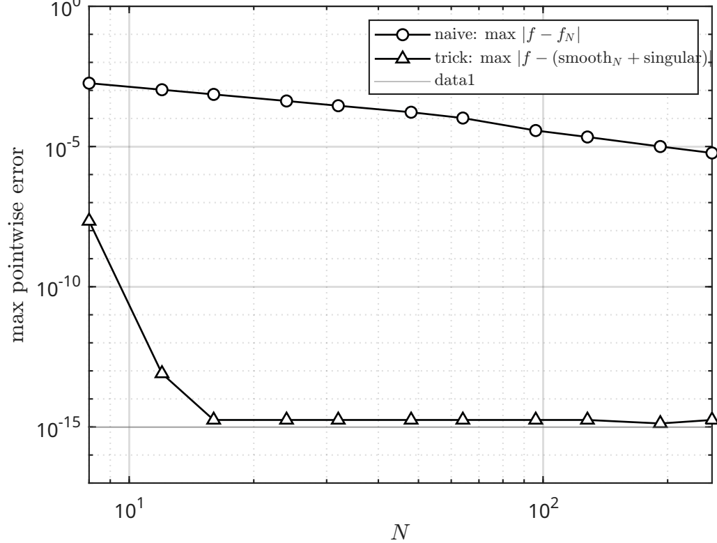
subtraction reaches machine \epsilon at modest N
