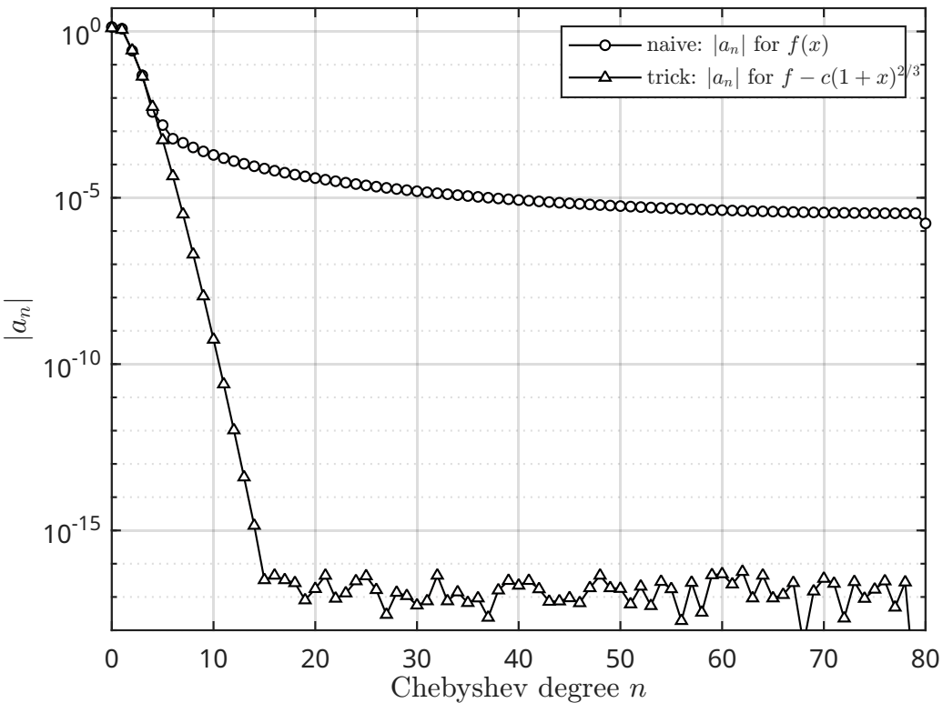
coefficient decay at N = 80
