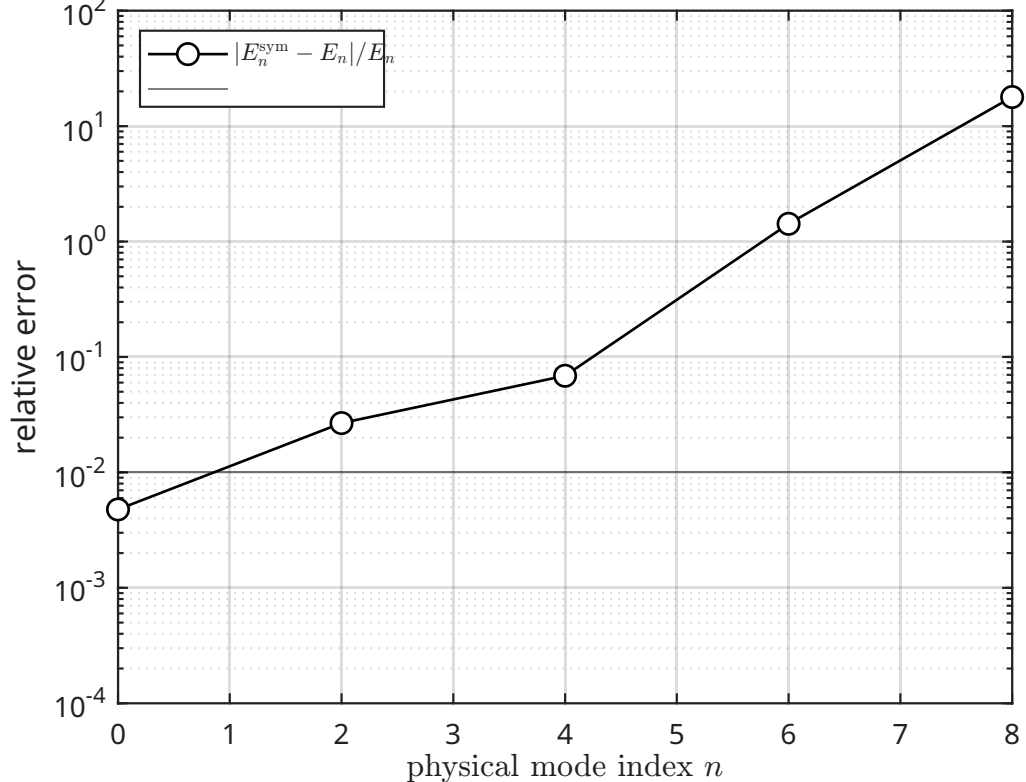
trust the lower spectrum: bottom 3 modes good, top 2 unusable
