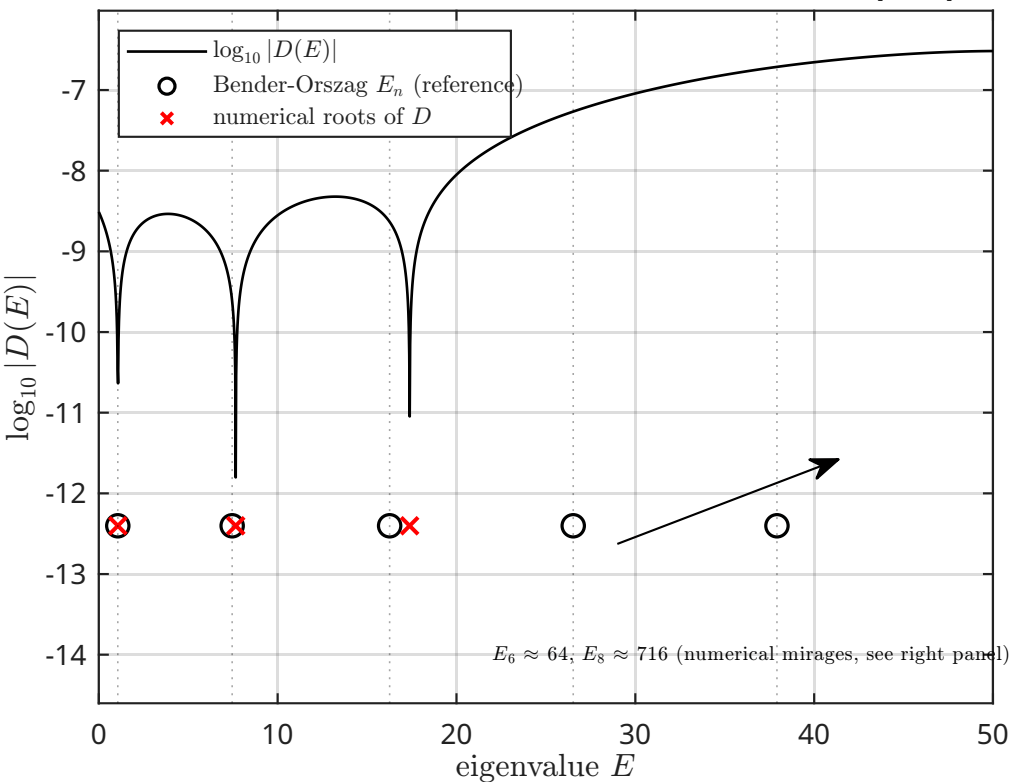
secular determinant zeros on the lower window E \in [0, 50]
