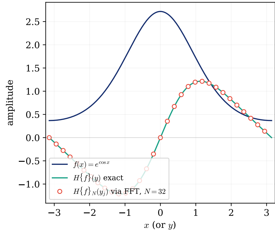
f(x) = e^{\cos x} and its Hilbert transform on the circle
