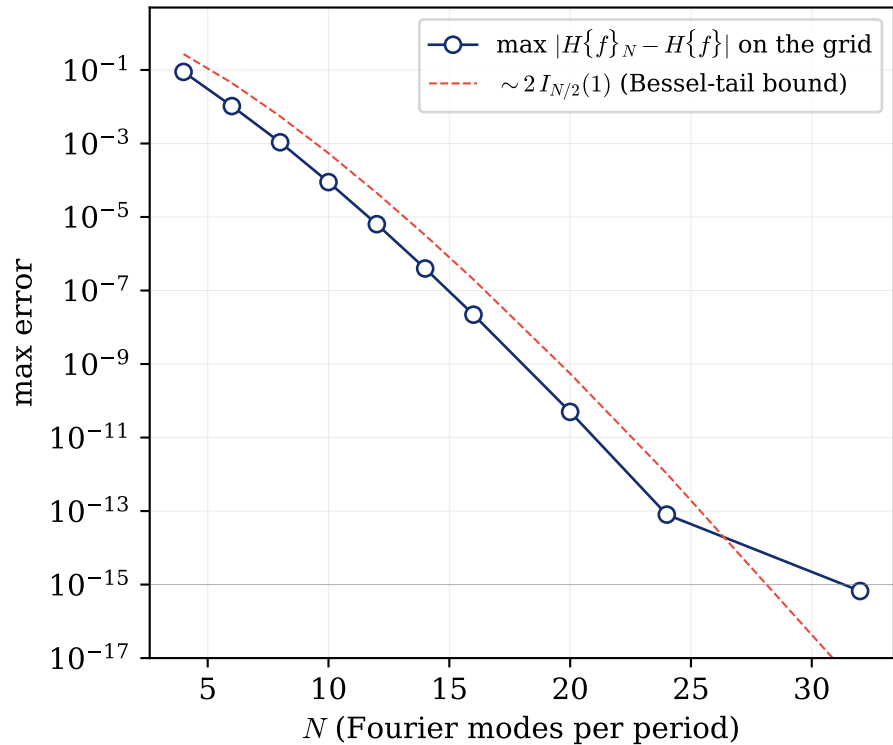
super-geometric convergence on a periodic analytic test
