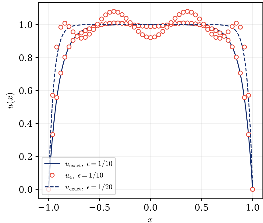
\epsilon^2 u'' - u = -1, u(\pm 1) = 0 : four-term Galerkin vs exact
