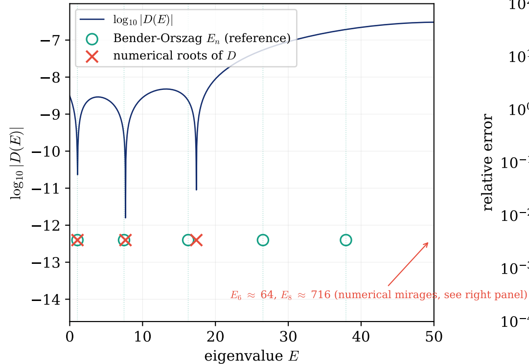
secular determinant zeros on the lower window E \in [0, 50]
