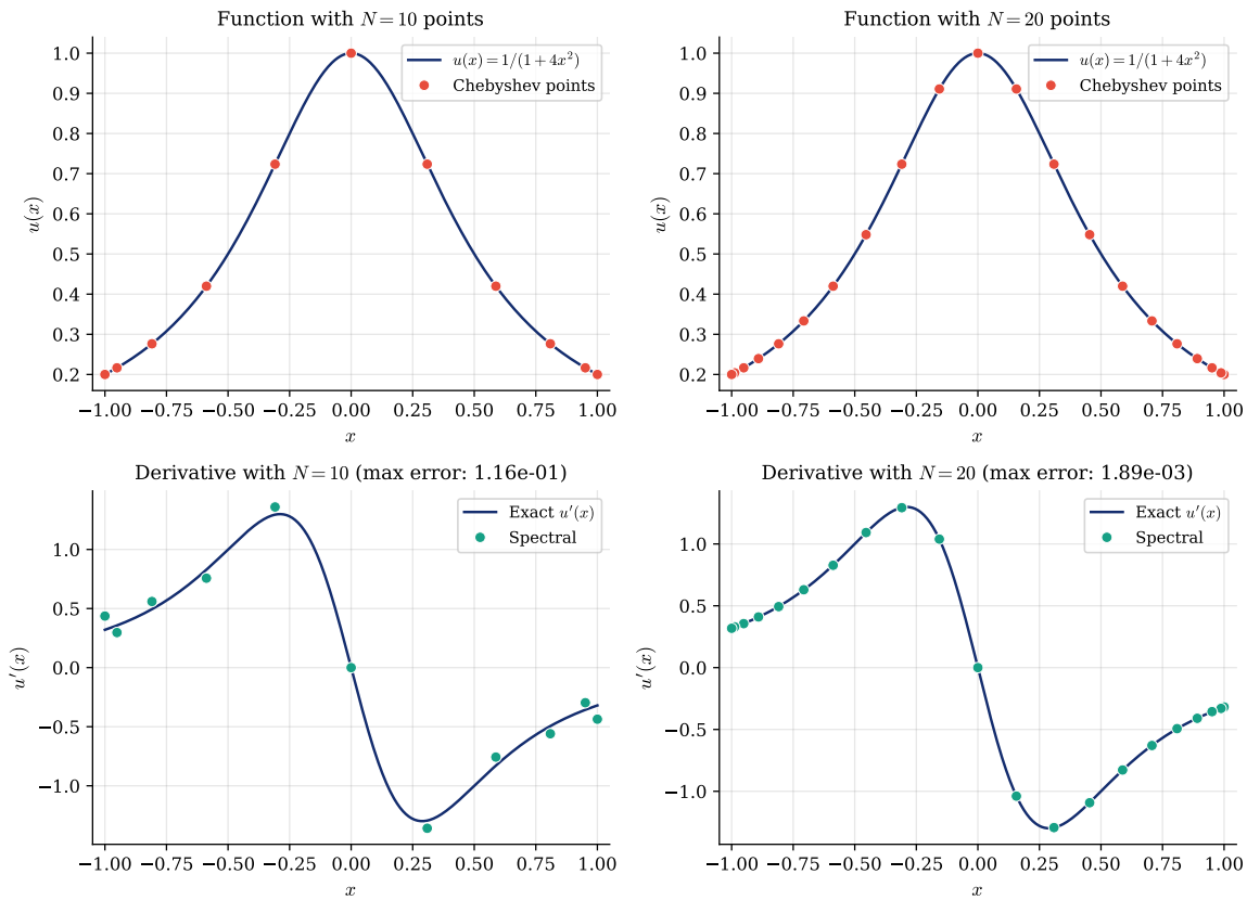
Figure 35: Chebyshev spectral differentiation of the Witch of Agnesi u(x) = 1/(1 + 4x^2) . Top row: function values at Chebyshev points. Bottom row: comparison of exact and spectral derivatives, with maximum errors indicated. The error decreases exponentially with N .
