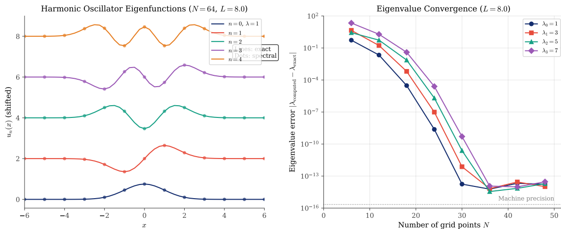
Figure 45: The quantum harmonic oscillator eigenvalue problem. Left: First five eigenfunctions computed with N = 64 Chebyshev points on [-8, 8] (dots) compared to exact Hermite functions (lines). Right: Eigenvalue error versus N for the first four eigenvalues. The error decreases faster than any exponential, reaching machine precision around N = 36 .
