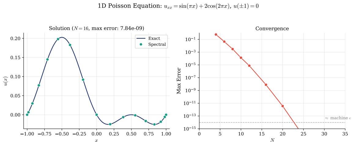
Figure 37: Solution of the 1D Poisson equation Equation 66. Left: numerical solution (circles) compared with exact solution (line) for N = 16 . Right: exponential convergence of the maximum error, reaching machine precision by N = 24 .
