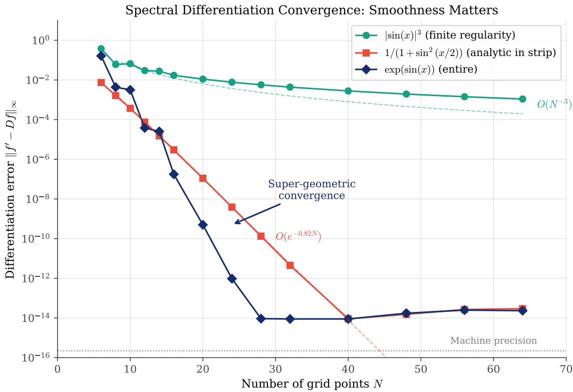
Figure 31: Spectral differentiation convergence rates for three functions of increasing smoothness. The error is measured in the maximum norm \|f' - Df\|_\infty . Functions with greater smoothness achieve faster convergence, exactly as predicted by Theorem 4.
