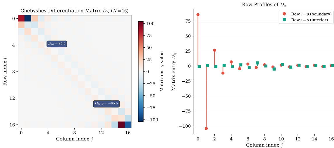
Figure 33: Structure of the Chebyshev differentiation matrix for N = 16 . Left: heatmap showing the matrix entries, with red indicating positive values and blue indicating negative. The large corner entries (D_N)_{00} and (D_N)_{NN} are visible. Right: row profiles showing boundary row (red) and interior row (green). The boundary row has large entries reflecting the O(N^2) corner values.
