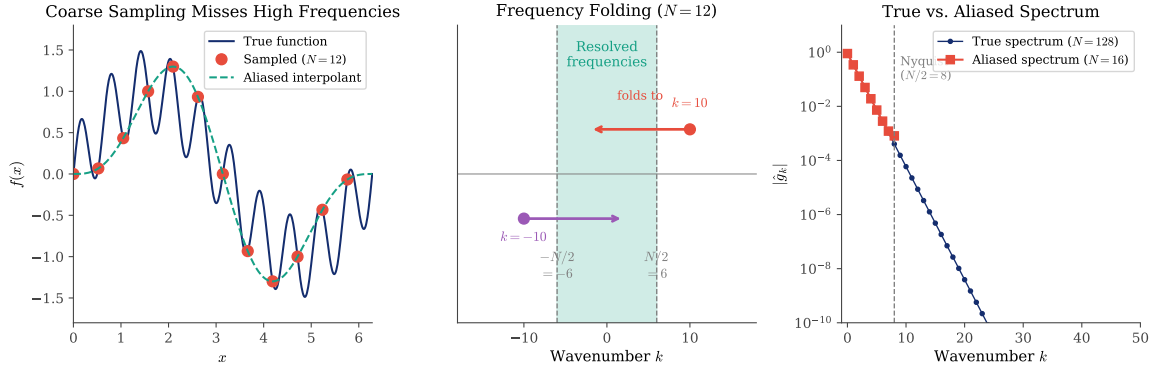
Figure 30: The aliasing phenomenon. Left: A function f(x) = \sin(x) + 0.5 \sin(10x) sampled at N = 12 points. The high-frequency component \sin(10x) aliases to \sin(-2x) , producing a misleading interpolant. Center: Frequency folding diagram showing how wavenumbers k = 10 and k = -10 fold into the resolved range [-6, 6] . Right: True versus aliased spectrum for f(x) = 1/(1.5 + \cos(x)) .
