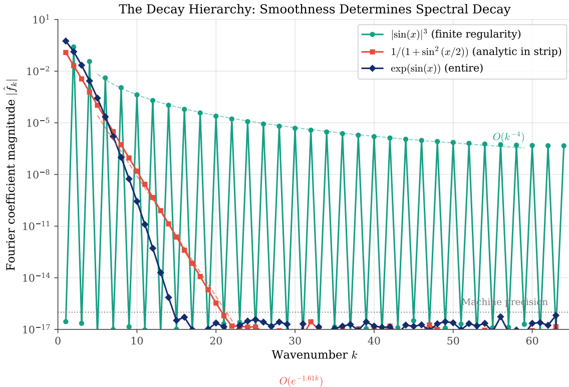
Figure 29: The decay hierarchy of Fourier coefficients. Functions with greater smoothness exhibit faster decay: algebraic ( O(k^{-4}) ) for finite regularity, geometric ( O(e^{-\alpha k}) ) for strip-analytic functions, and super-geometric for entire functions. The plot shows |\hat{f}_k| versus wavenumber k on a semi-log scale.
