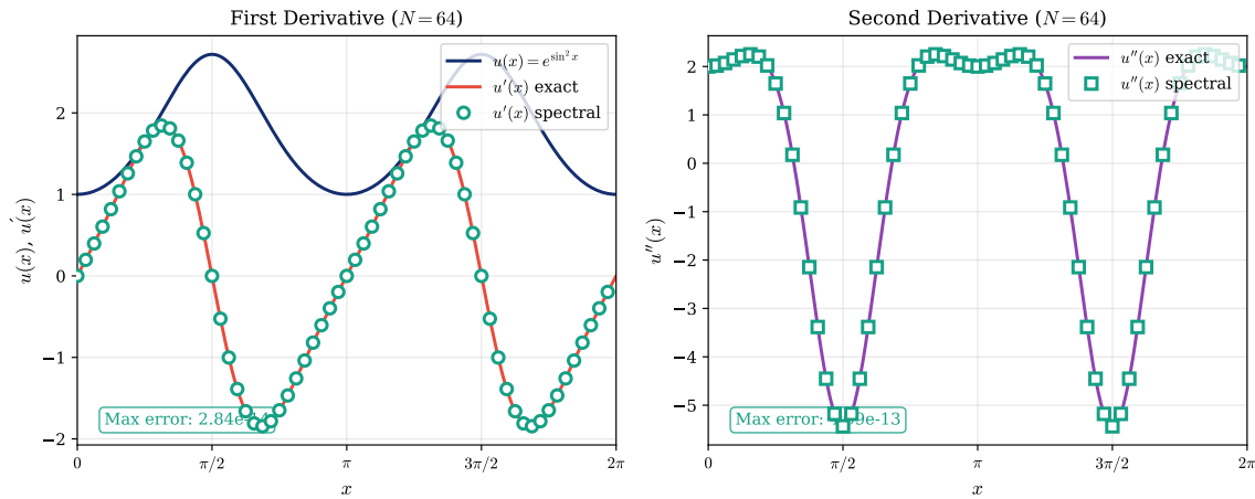
Figure 24: Spectral differentiation of u(x) = e^{\sin^2 x} using N = 64 grid points. Left: the function u (navy) and its first derivative u' exact (coral) vs. spectral (teal circles). Right: second derivative u'' exact (purple) vs. spectral (teal squares). The maximum errors, displayed in each panel, are near machine precision ( \approx 10^{-14} ). This remarkable accuracy with relatively few points is the hallmark of spectral methods for smooth periodic functions.
