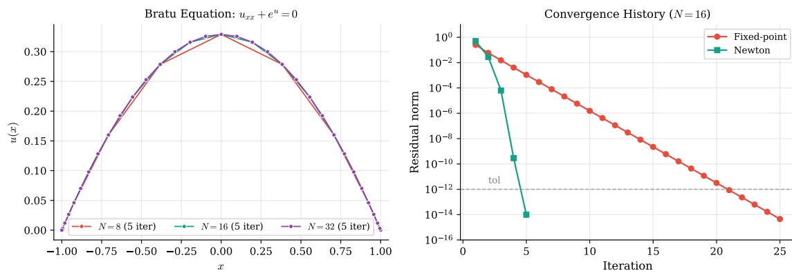
Figure 39: Nonlinear BVP: the Bratu equation Equation 70 with \lambda = 0.5 . Left: solutions for different values of N . Right: convergence history comparing Newton iteration (quadratic convergence) with fixed-point iteration (linear convergence). Newton typically converges in 5–8 iterations.
