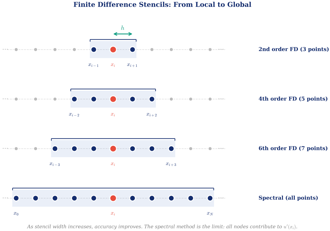
Figure 20: Finite difference stencils in one dimension, progressing from local to global. The derivative at the central node x_i (red) is approximated using only the highlighted nodes (blue) within each stencil. From top to bottom: 3-point stencil (2nd order), 5-point stencil (4th order), 7-point stencil (6th order), and spectral method (all nodes). As the stencil widens, accuracy improves. The spectral method represents the limiting case where every node contributes to the derivative approximation, yielding exponential rather than algebraic convergence.
