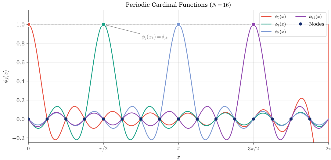
Figure 22: Periodic cardinal functions \varphi_j(x) for N = 16 equispaced nodes on [0, 2\pi) . Each function peaks at value 1 at its corresponding node x_j and vanishes at all other nodes, satisfying the cardinal property \varphi_j(x_k) = \delta_{jk} . The oscillations decay smoothly away from each peak, in contrast to the boundary-amplified oscillations seen in Lagrange basis polynomials for non-periodic interpolation.
