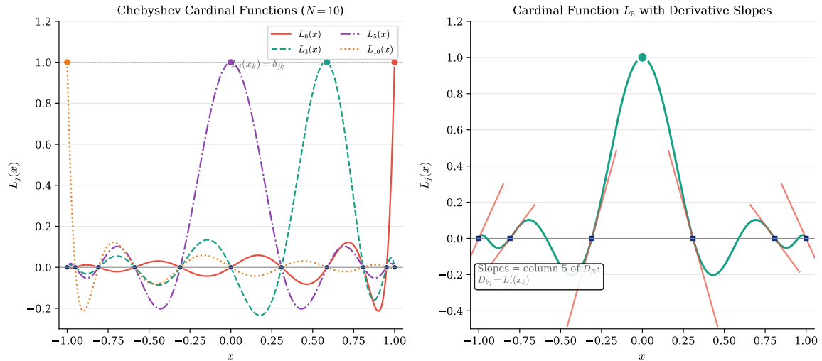
Figure 34: Chebyshev cardinal functions (Lagrange basis polynomials). Left: several cardinal functions for N = 10 , each peaking at value 1 at its corresponding node and vanishing at all others. Right: a single cardinal function with tangent lines at the grid points—the slopes of these tangent lines are precisely the entries in the corresponding column of the differentiation matrix.
