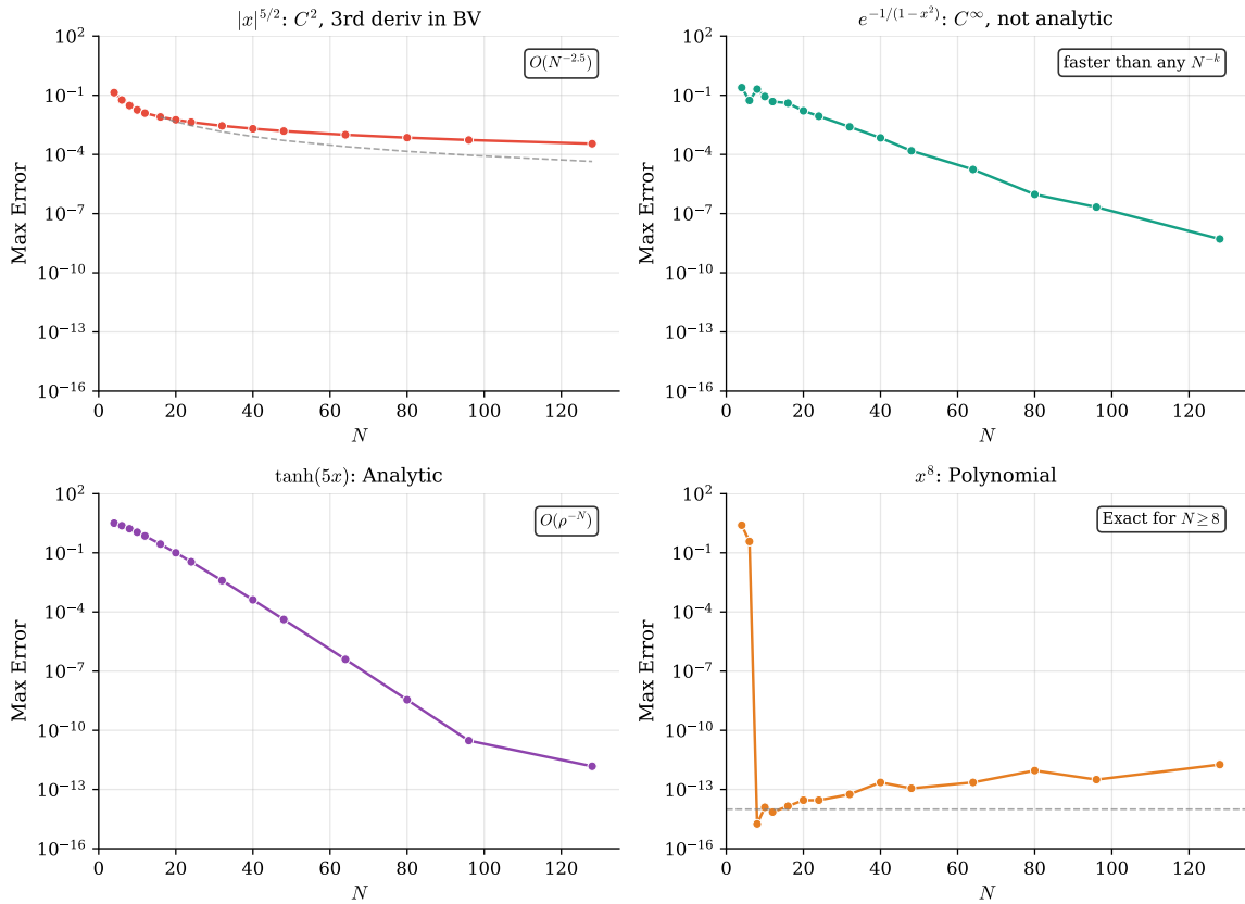
Figure 36: Convergence of the spectral differentiation error \|D_N v - u'(x)\|_\infty as a function of N for four test functions. Top left: |x|^{5/2} shows algebraic convergence O(N^{-2.5}) due to limited smoothness (Hölder regularity 5/2 ). Top right: the bump function e^{-1/(1-x^2)} achieves superalgebraic (faster than any power) but not exponential convergence, consistent with C^\infty but non-analytic behavior. Bottom left: \tanh(5x) demonstrates exponential convergence until machine precision, as expected for analytic functions. Bottom right: the polynomial x^8 is differentiated exactly for N \geq 8 .
