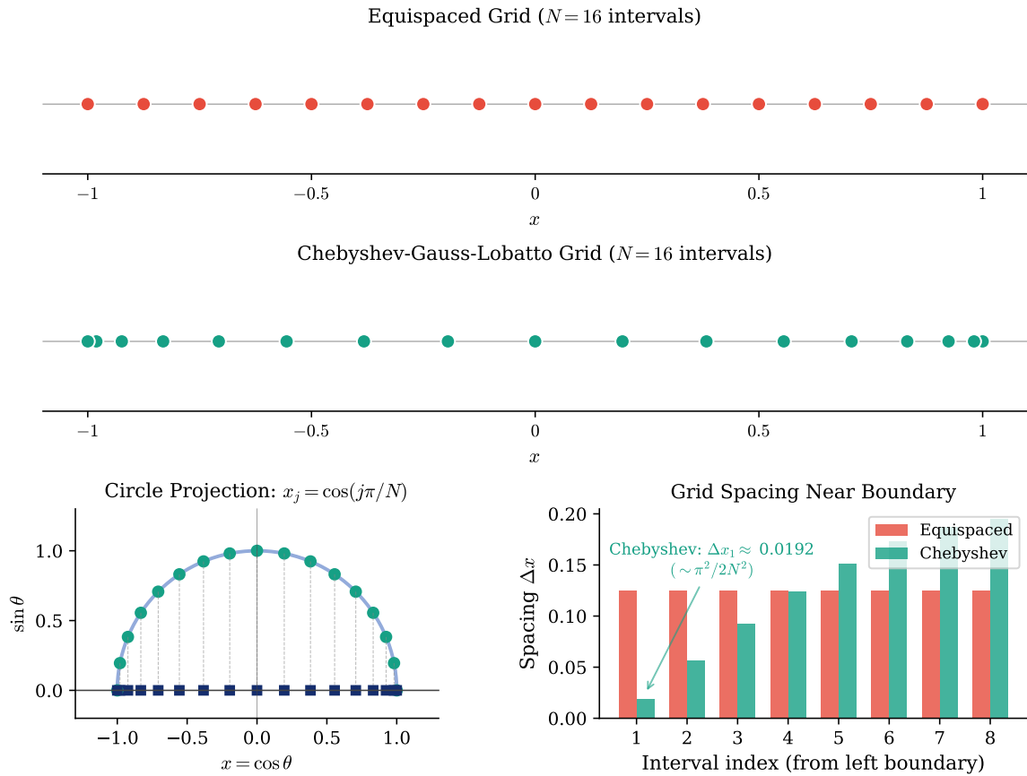
Figure 32: Comparison of equispaced and Chebyshev-Gauss-Lobatto grids for N = 16 intervals. Top: equispaced points are distributed uniformly. Middle: Chebyshev points cluster near the boundaries. Bottom left: the circle projection interpretation: Chebyshev points are the projections of equally-spaced points on a semicircle. Bottom right: comparison of grid spacing near the left boundary, showing the O(N^{-2}) clustering of Chebyshev points.
