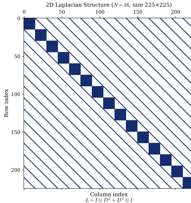
Figure 43: Sparsity pattern of the 2D Laplacian matrix for N = 16 . The (N - 1)^2 \times (N - 1)^2 matrix shows the characteristic block structure arising from the Kronecker product formulation Equation 73.
