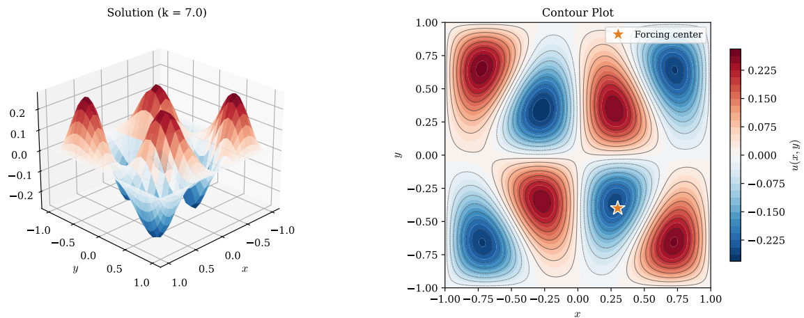
Figure 44: Helmholtz equation Equation 75 with k = 7 , near resonance with the (2,4) eigenmode ( k_{2,4} \approx 7.02 ). Left: 3D surface showing the wave-like structure. Right: contour plot with forcing location marked. The solution exhibits the characteristic pattern of the (2,4) eigenmode.
