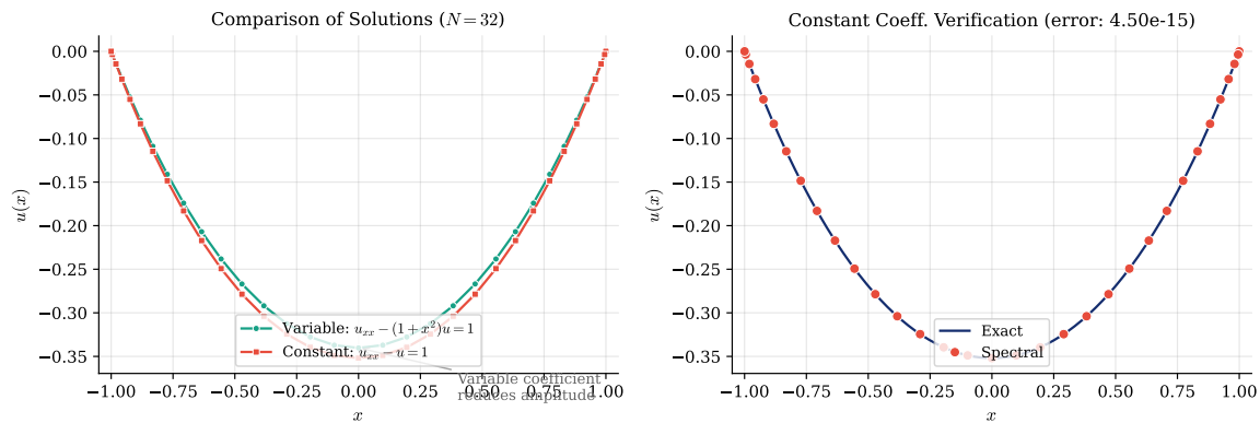
Figure 38: Variable coefficient BVP Equation 68. Left: comparison of solutions for variable coefficient (1 + x^2) and constant coefficient (1) . The variable coefficient reduces the solution amplitude, especially near the boundaries where 1 + x^2 is largest. Right: verification of the constant-coefficient case against its exact solution.
