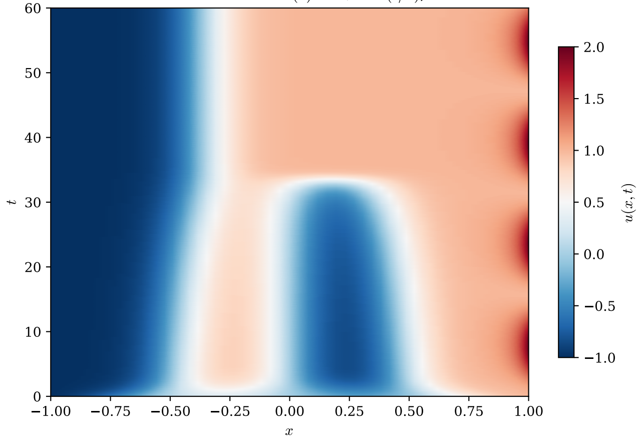
Allen-Cahn: Driven BC u(1) = 1 + \sin^2(t/5) , \varepsilon = 0.01
