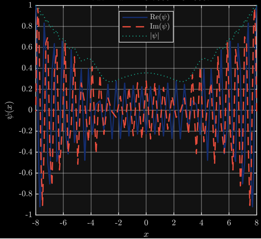
Mode 2: \omega = -9.7068 - 0.2068i
