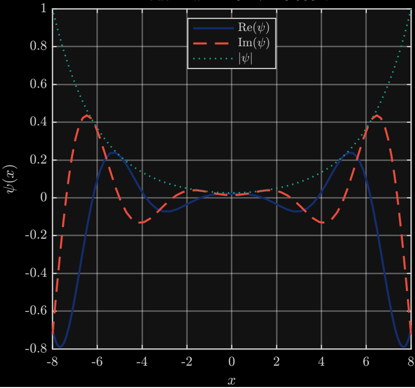
Mode 1: \omega = 1.3227 - 0.5002i
