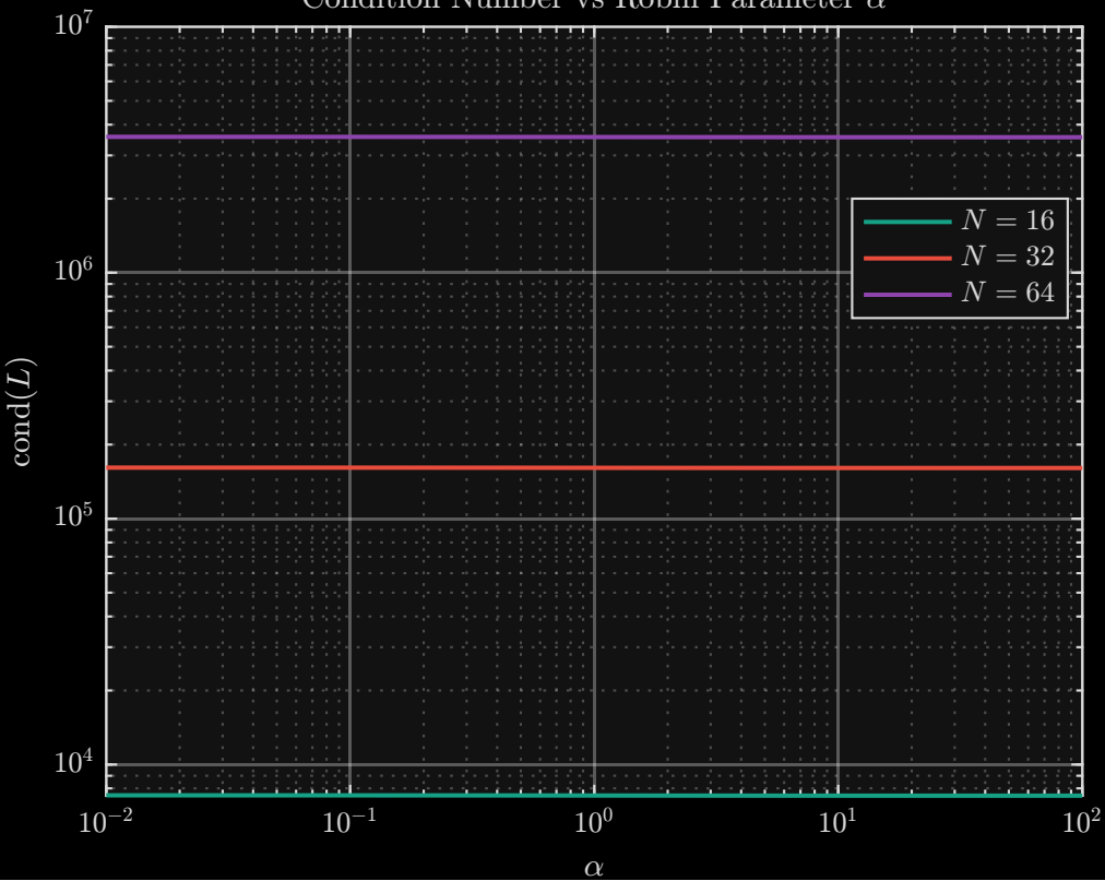
Condition Number vs Robin Parameter \alpha
