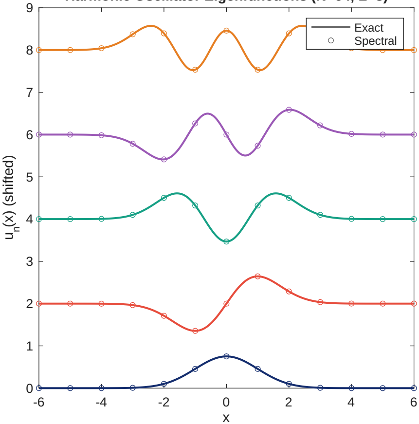
Harmonic Oscillator Eigenfunctions (N=64, L=8)
