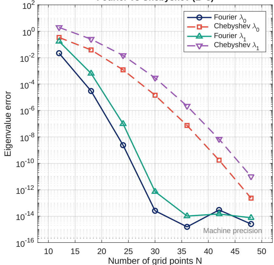
Fourier vs Chebyshev (L=8)
