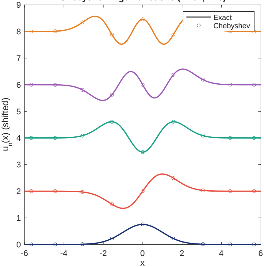
Chebyshev Eigenfunctions (N=64, L=8)
