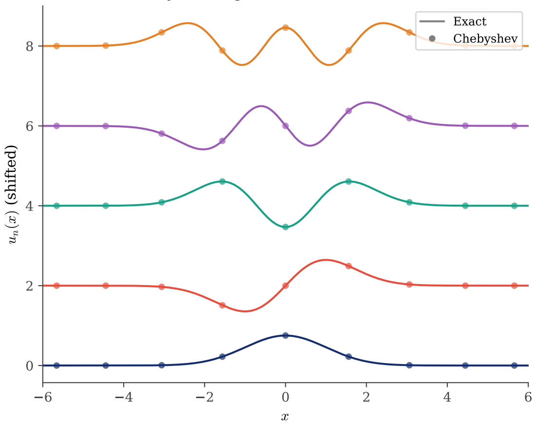
Chebyshev Eigenfunctions ( N = 64 , L = 8 )
