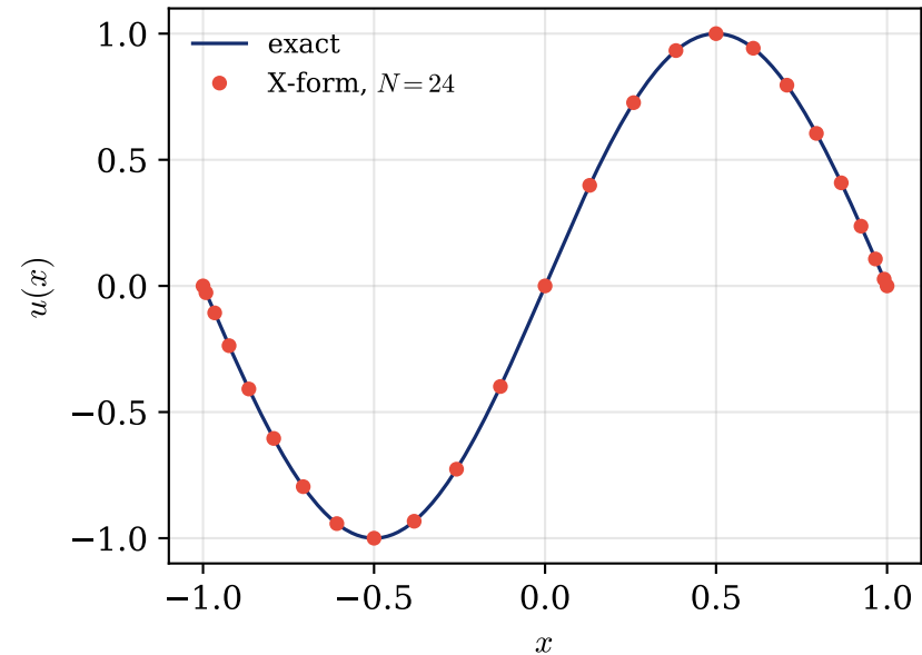
(a) Manufactured BVP
