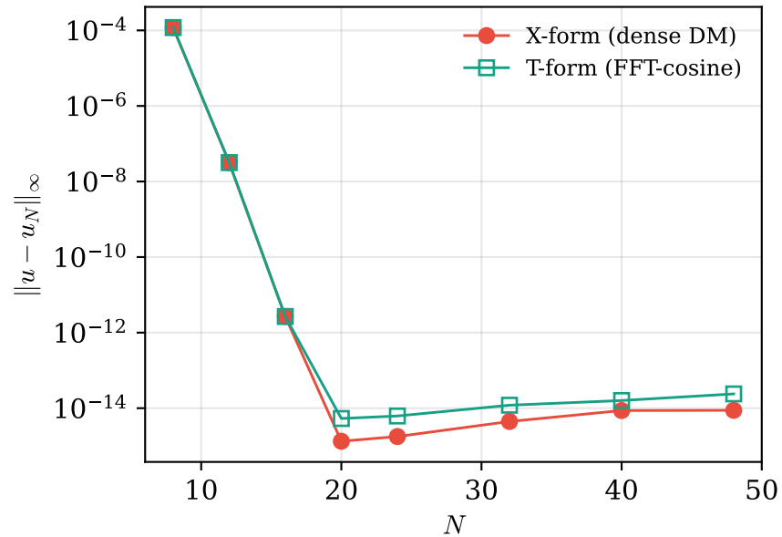
(b) Same convergence, different arithmetic
