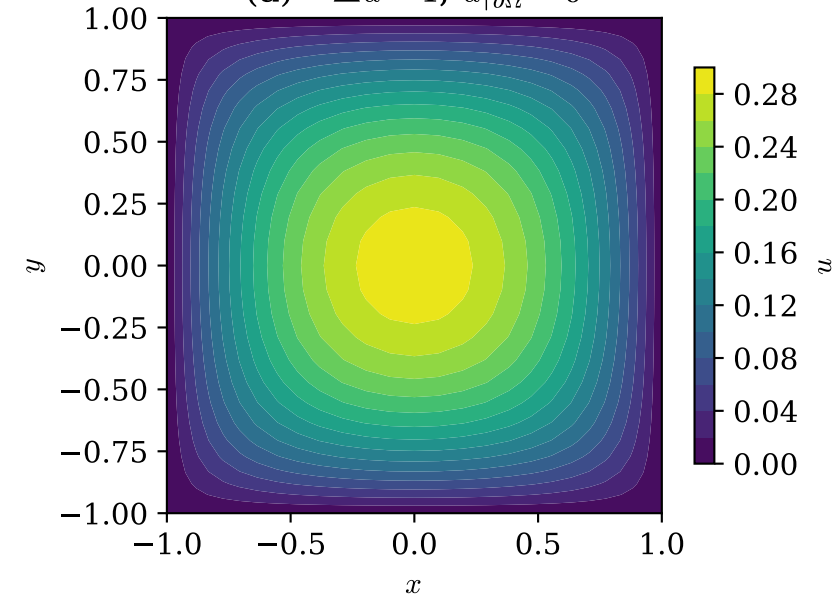
(a) -\Delta u = 1, u|_{\partial\Omega} = 0
