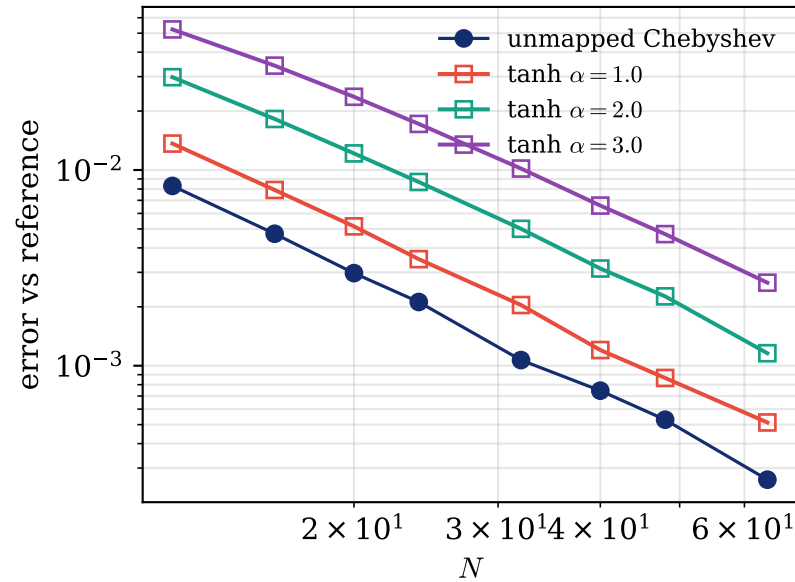
(c) Corner convergence
