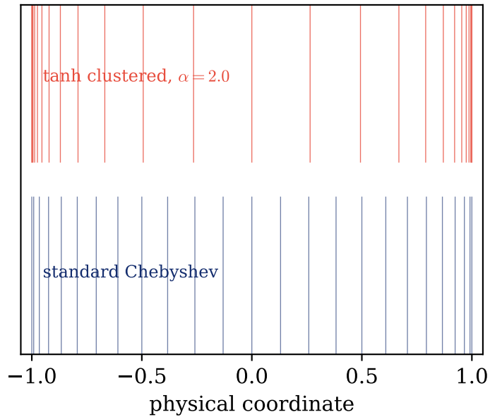
(b) Grids at N = 24
