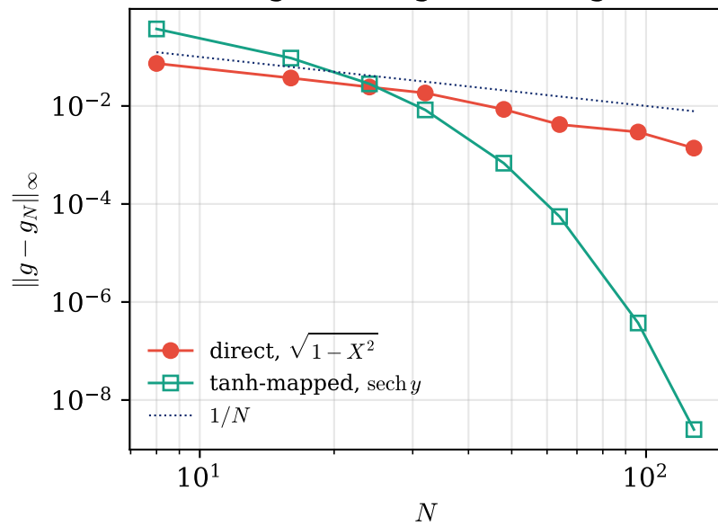
(b) Convergence: algebraic vs geometric
