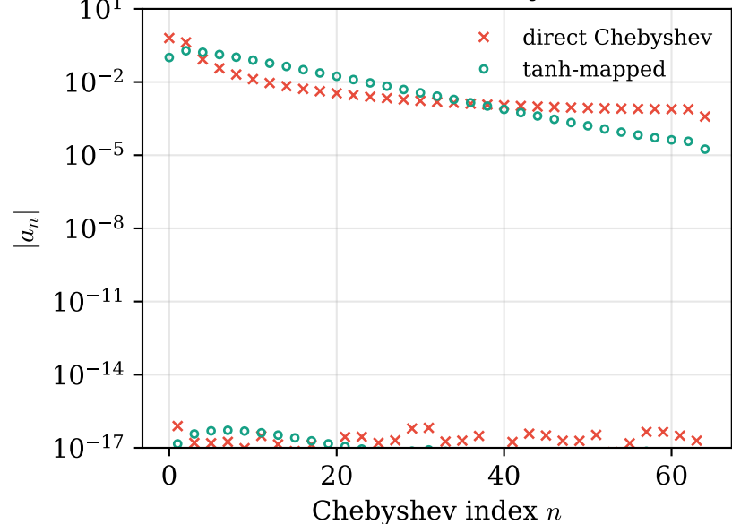
(c) Coefficient decay, N=64
