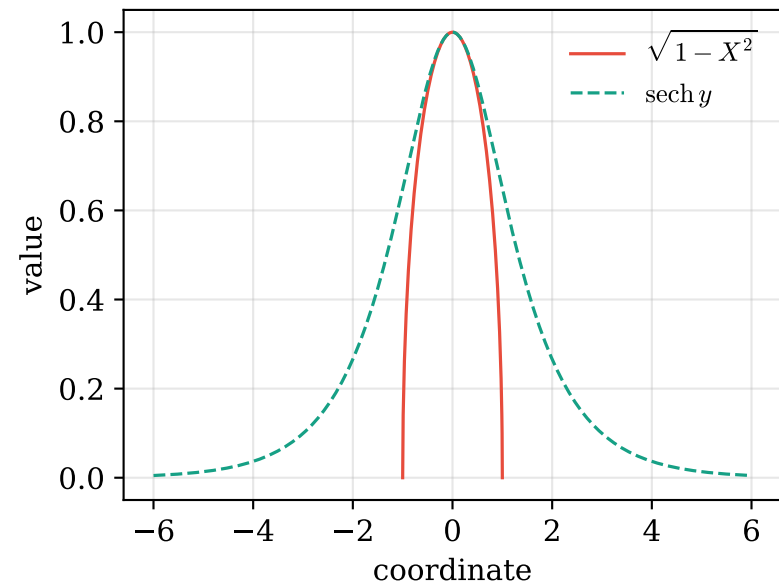
(a) Two views of the same function
