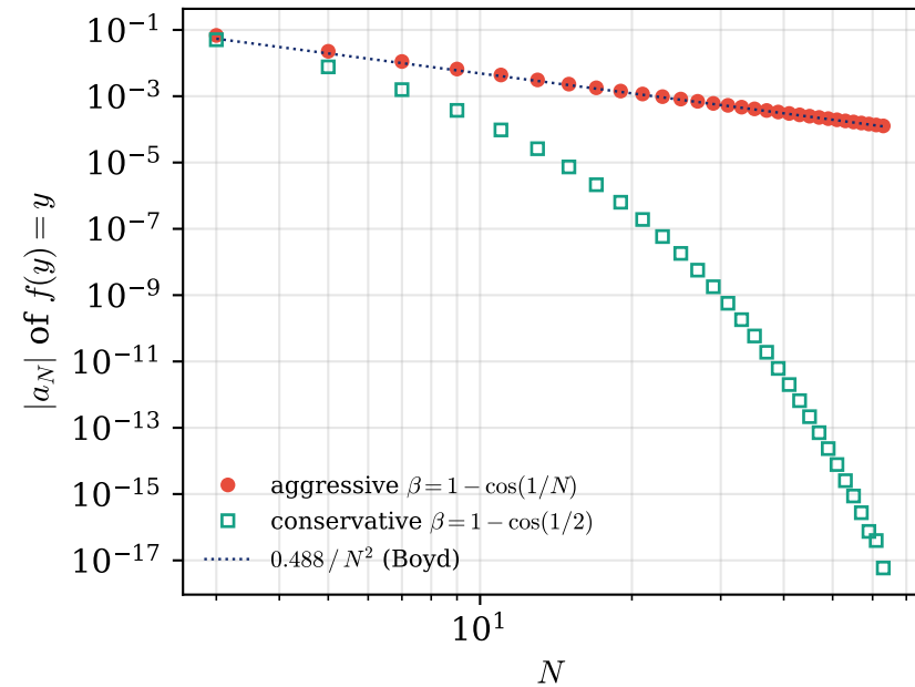
(c) Accuracy destroyed by aggressive scaling
