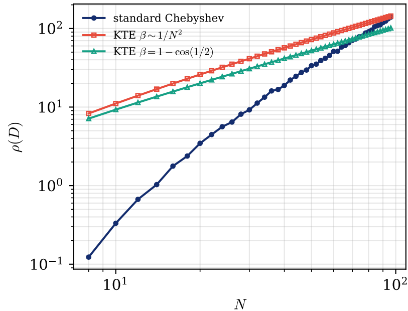
(b) Stiffness of first-derivative matrix
