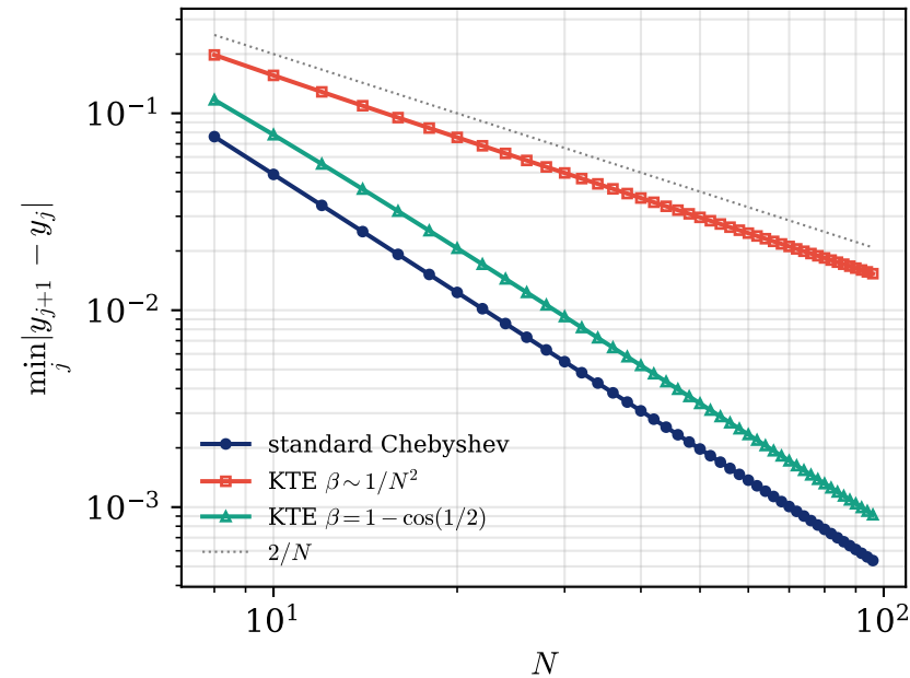
(a) Minimum spacing vs N
