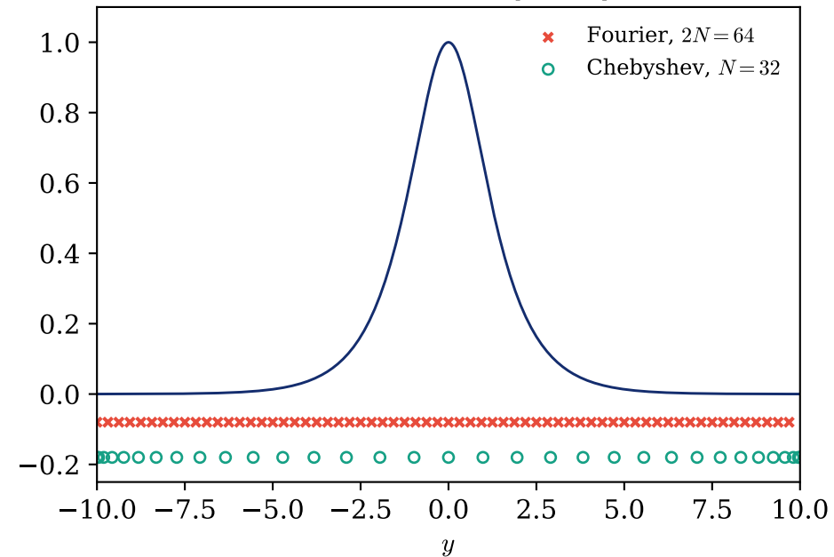
(a) Grid densities on [-L, L] , L = 10
