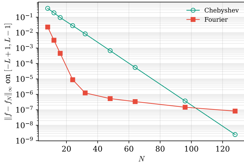
(b) Interior error at fixed L = 10
