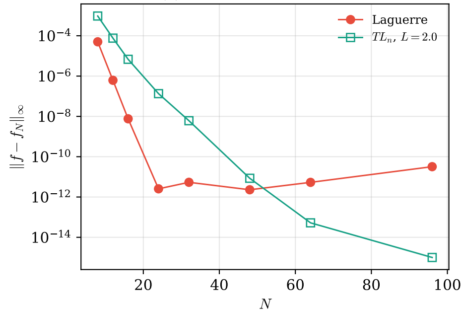
(a) f(y) = e^{-y} (exponential decay)
