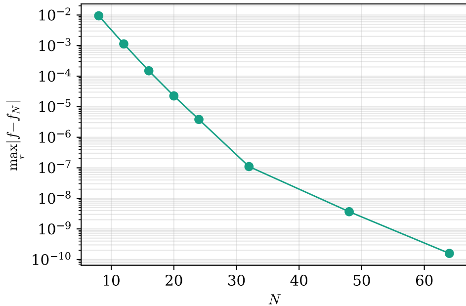
(b) Subgeometric descent, L=4.0
