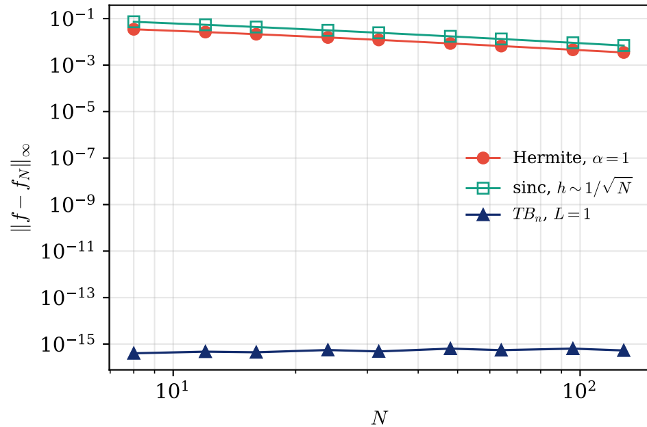
(b) Algebraic, subgeometric, geometric
