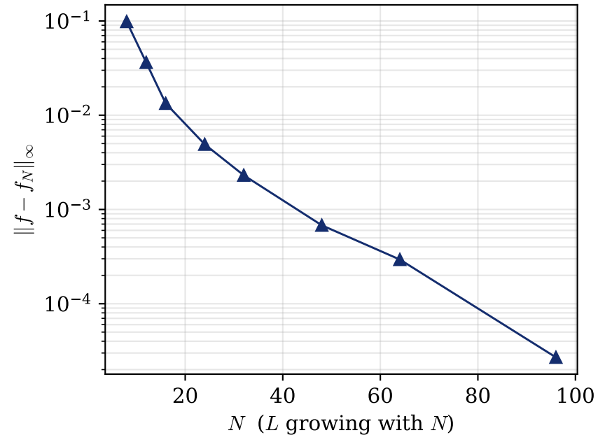
(c) Grow both: subgeometric descent
