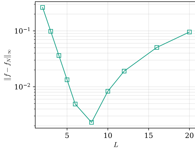
(b) Fix N=32 , vary L : sweet spot
