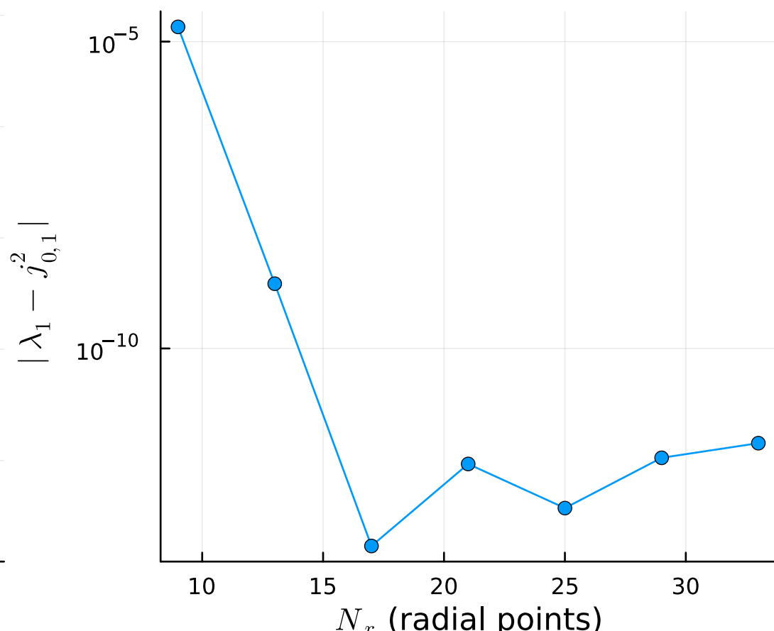
Exponential convergence
