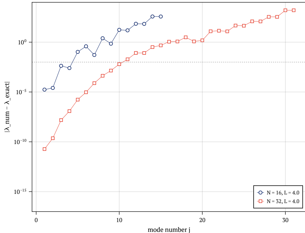
infinite-interval tax: oscillator spectrum
