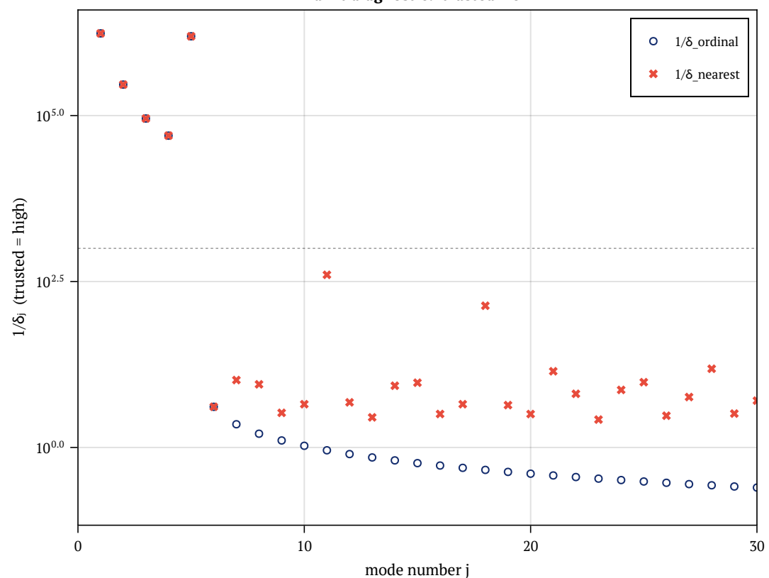
drift diagnostic: trusted = 5
