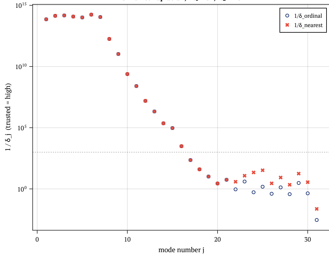
Dirichlet Laplacian, N_1 = 32, N_2 = 48
