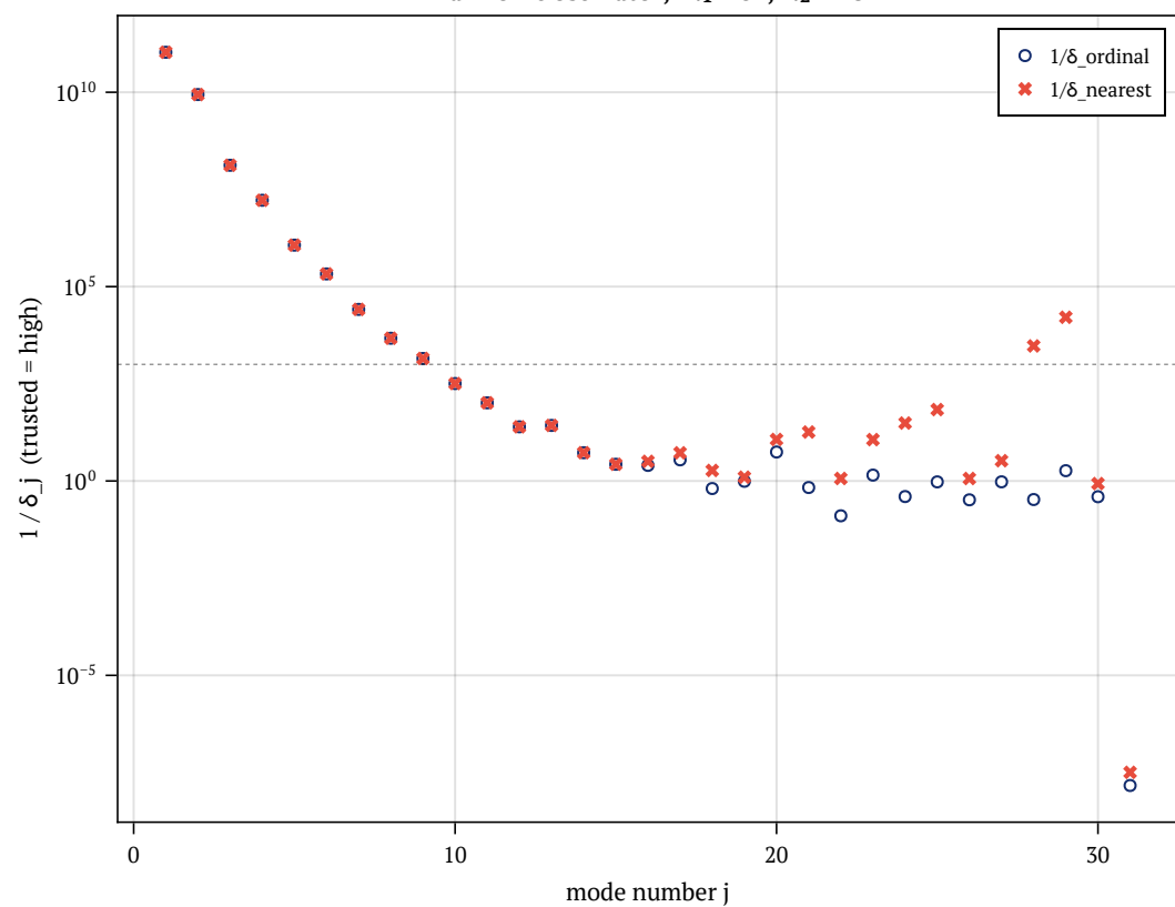
Harmonic oscillator, N_1 = 32, N_2 = 48
