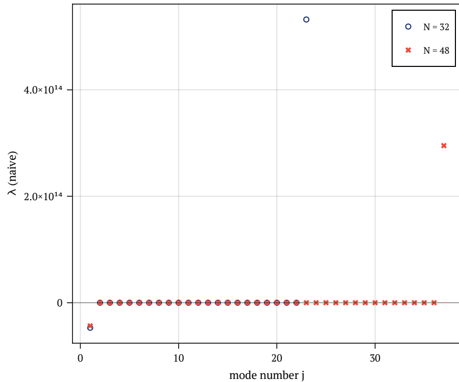
naive: spurious \lambda > 0 visible
