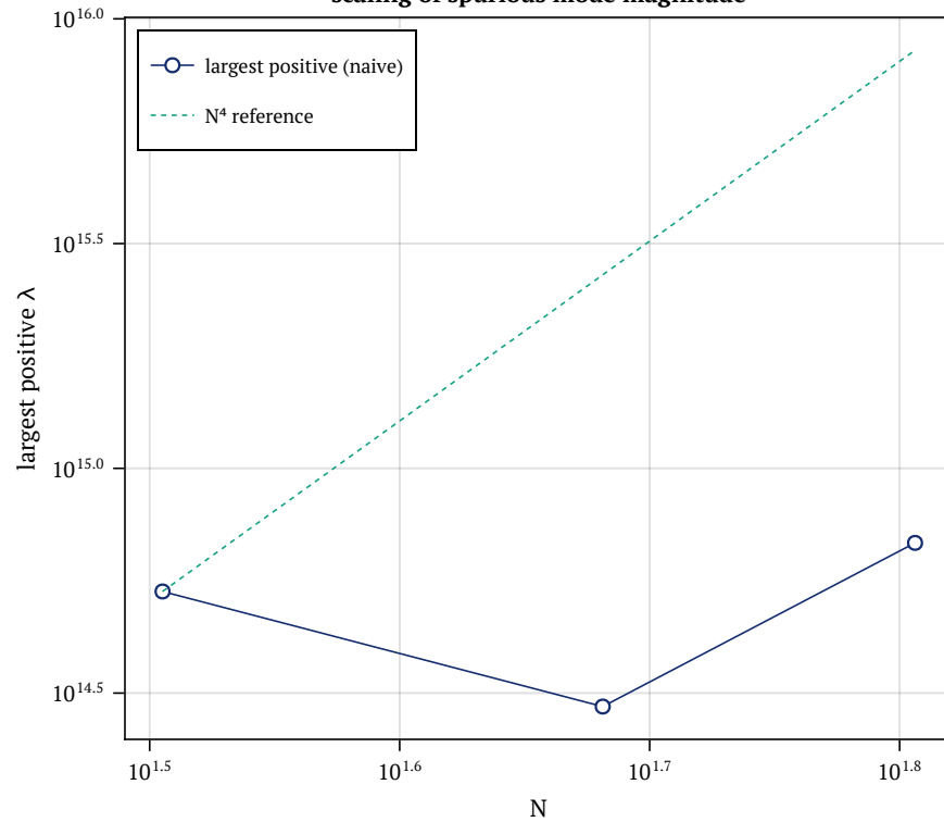
scaling of spurious mode magnitude
