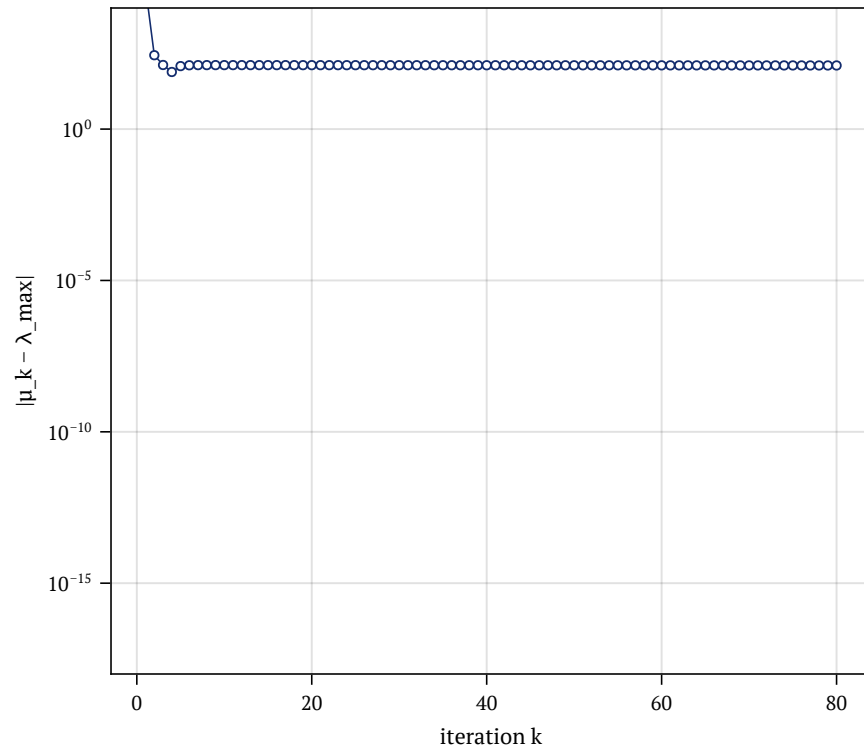
power method \rightarrow \lambda_{\max} = 49939.246
