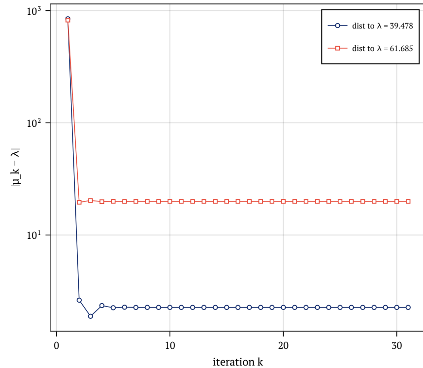
cautionary: \mu = 50.582 between two modes
