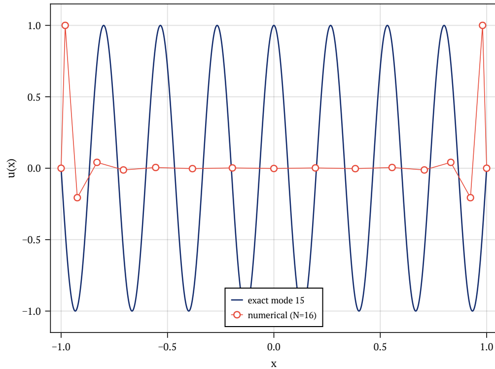
mode j=15: \lambda_{\text{num}}=3174.7923 , \lambda_{\text{exact}}=555.1652
