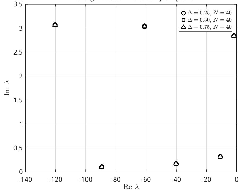
first eigenvalues in the complex plane
