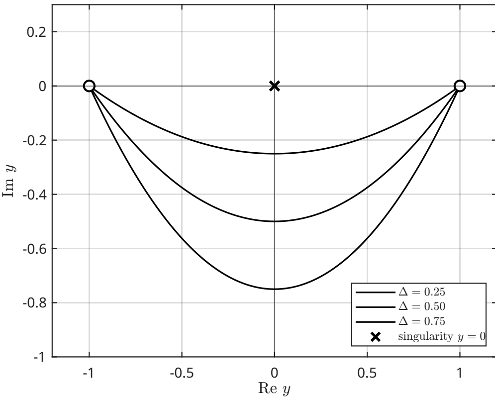
parabolic detour y(x) = x + i\Delta(x^2 - 1)
