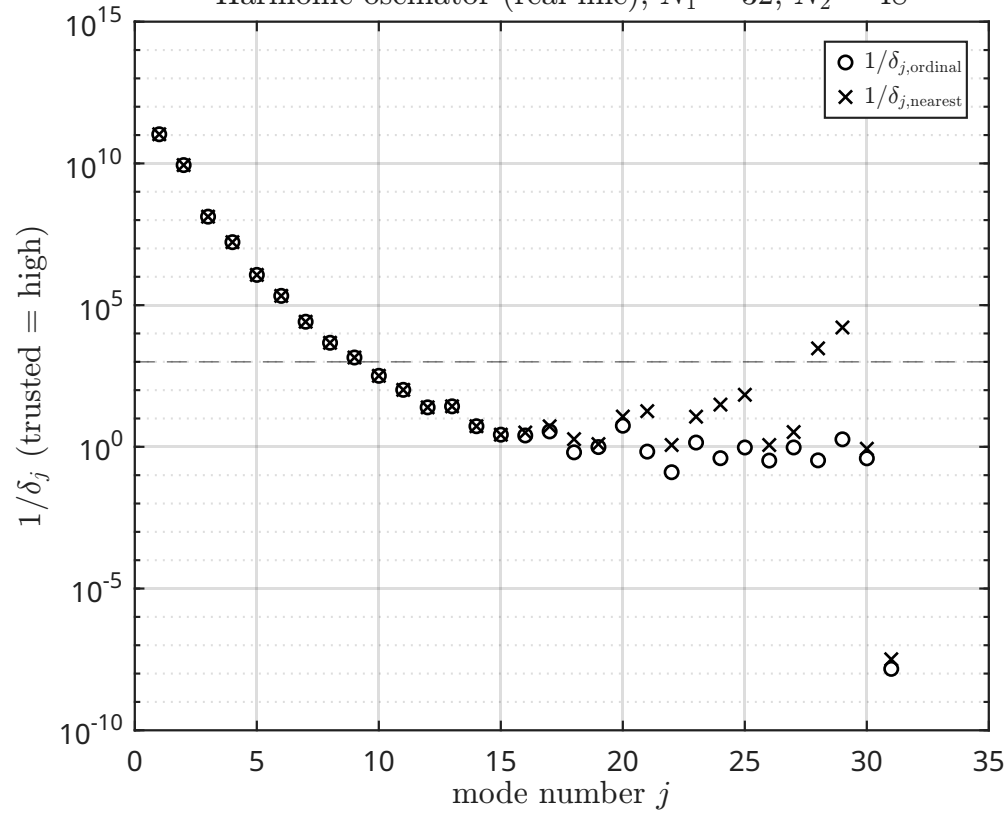
Harmonic oscillator (real line), N_1 = 32 , N_2 = 48
