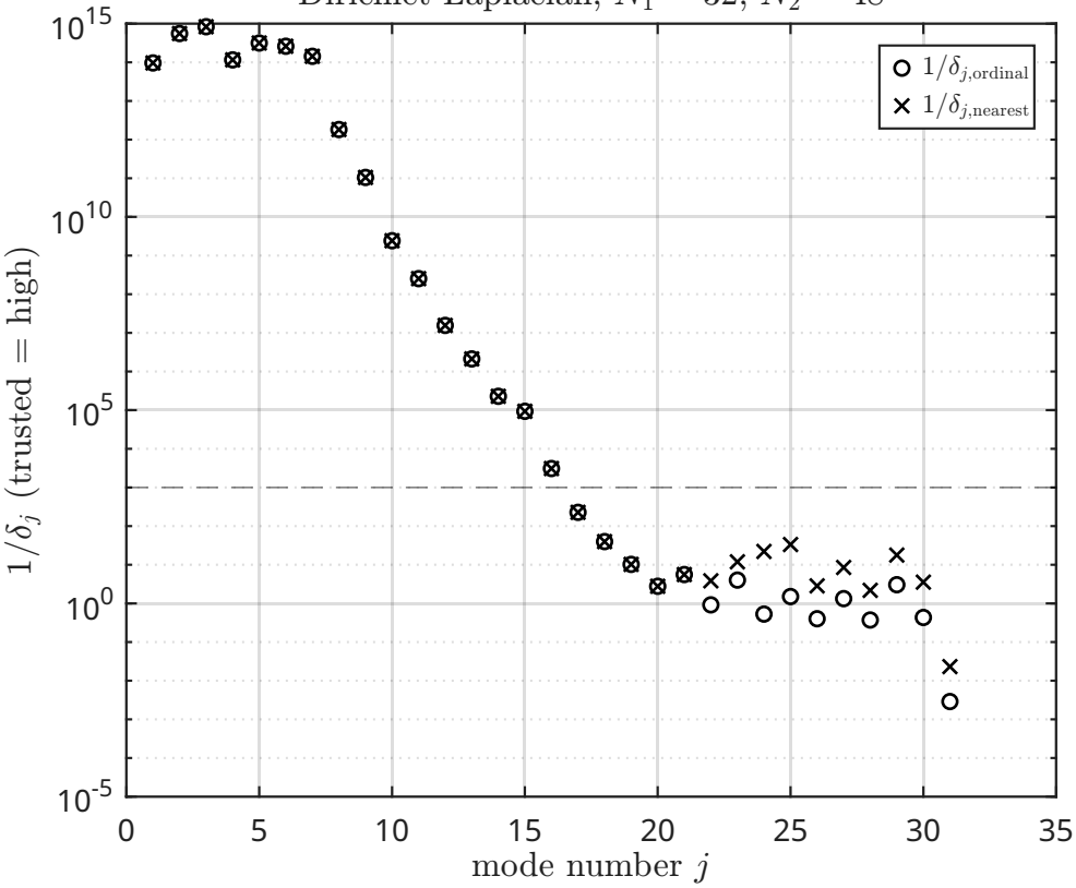
Dirichlet Laplacian, N_1 = 32 , N_2 = 48
