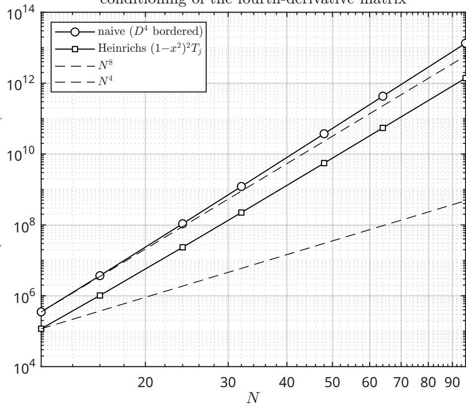
conditioning of the fourth-derivative matrix
