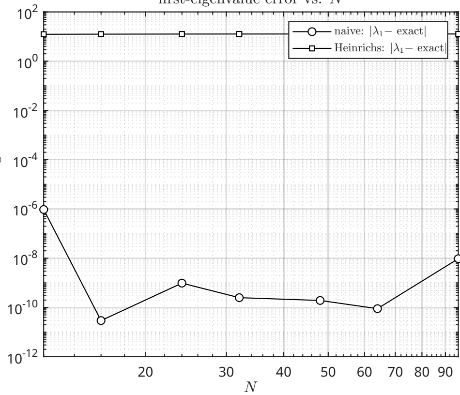
first-eigenvalue error vs. N
