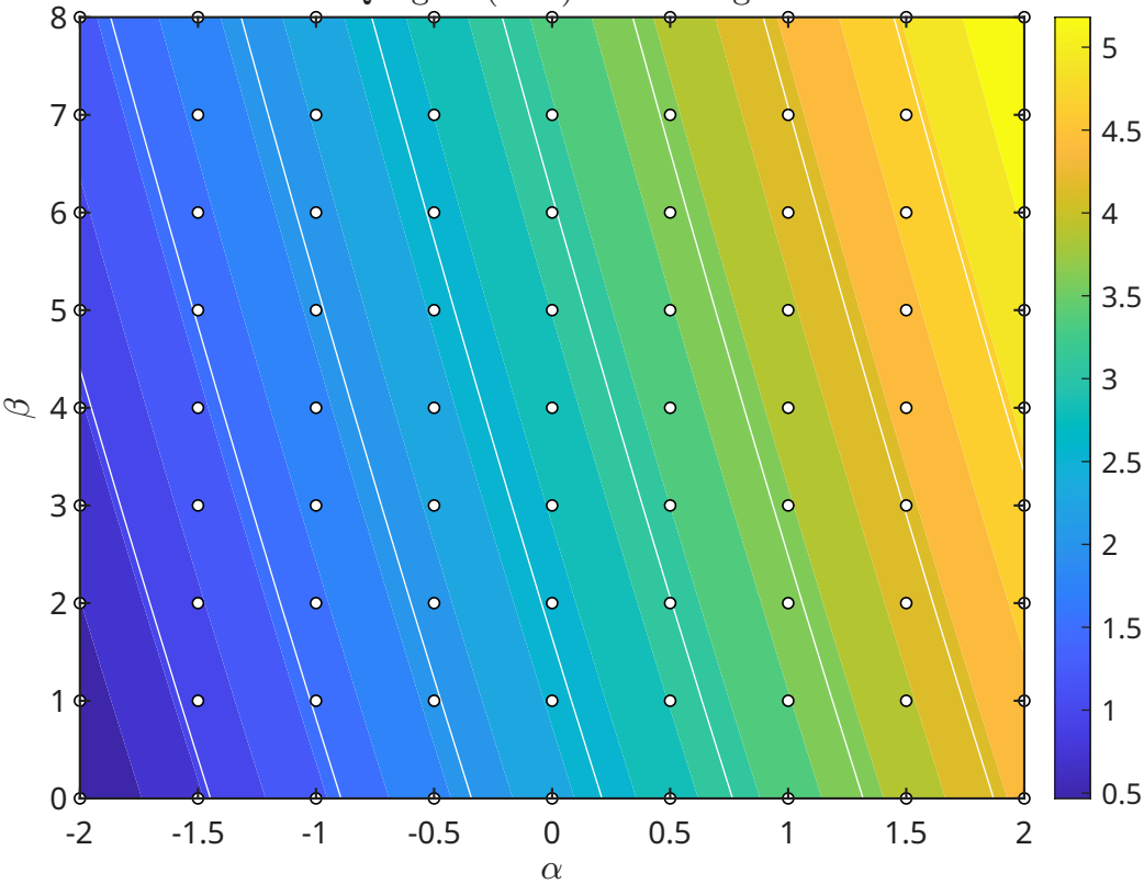
coarse QR grid ( 9 \times 9 ): lowest eigenvalue
