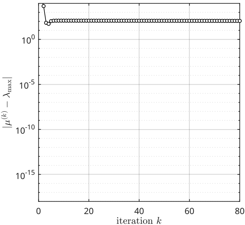
power method \rightarrow \lambda_{\max} = 49939.246
