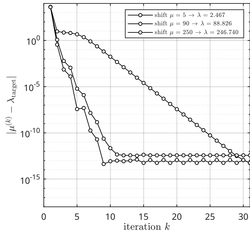
inverse iteration: three shifts, three modes
