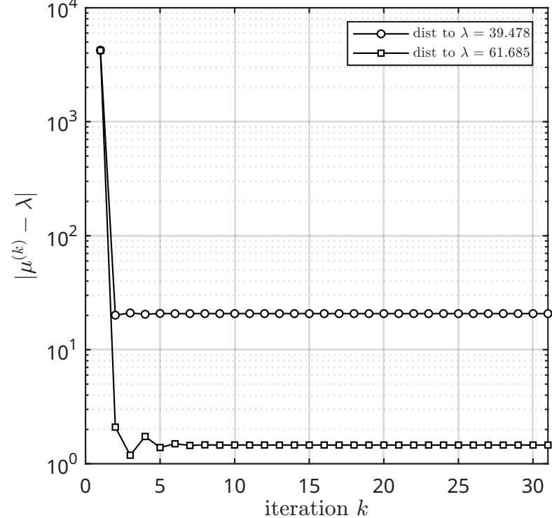
cautionary: \mu = 50.582 between two modes
