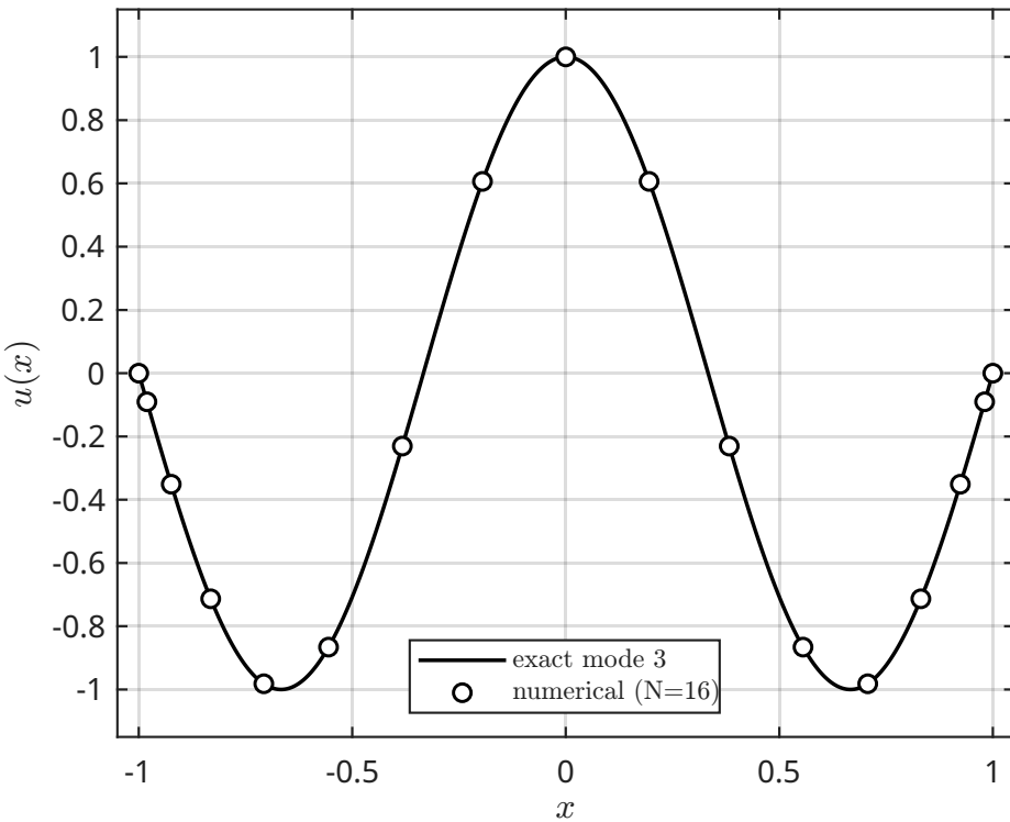
mode j = 3 : \lambda_{\text{num}} = 22.2066 , \lambda_{\text{exact}} = 22.2066
