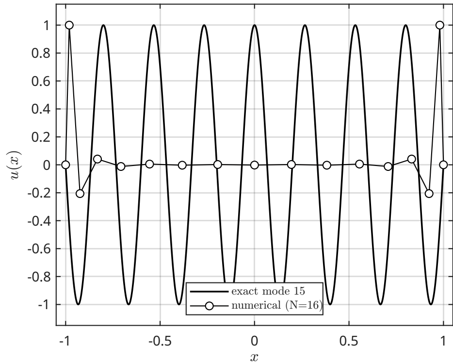
mode j = 15 : \lambda_{\text{num}} = 3174.7923 , \lambda_{\text{exact}} = 555.1652
