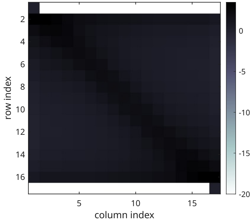
\log_{10} |A| for boundary-bordered pencil
