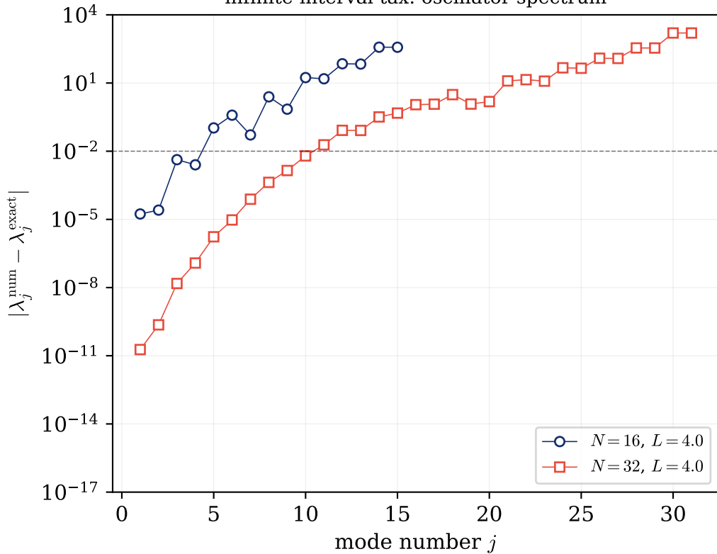
infinite-interval tax: oscillator spectrum
