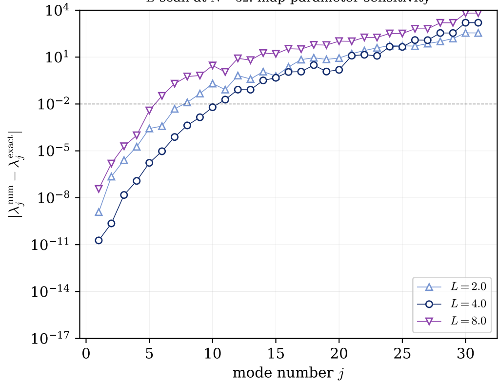
L -scan at N=32 : map-parameter sensitivity
