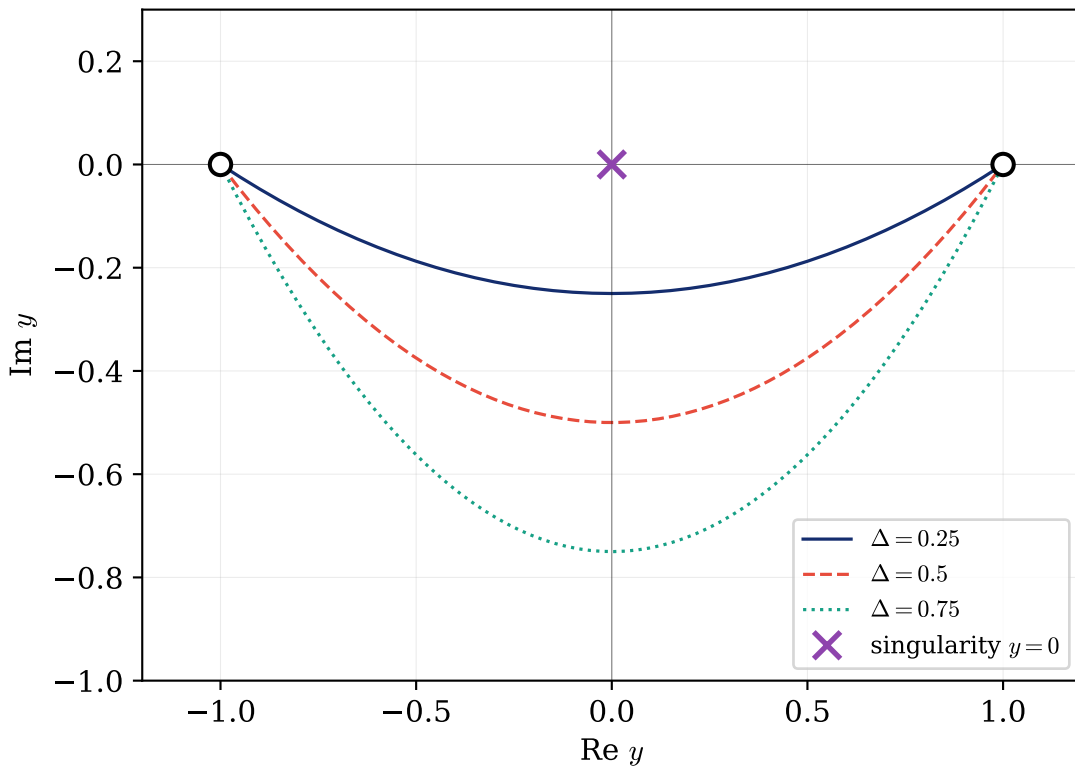
parabolic detour y(x) = x + i\Delta(x^2 - 1)
