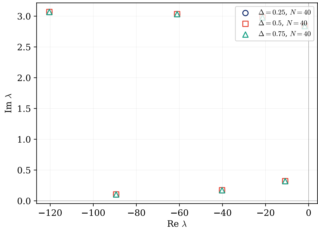
first eigenvalues in the complex plane
