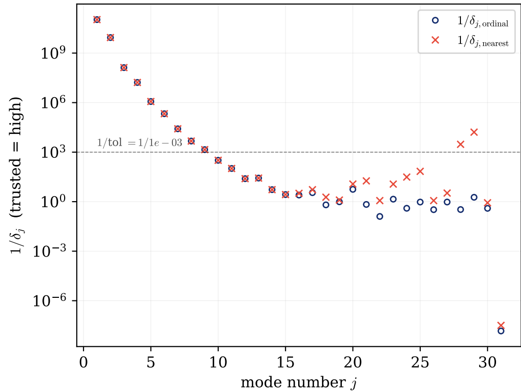
Harmonic oscillator (real line), N_1 = 32, N_2 = 48
