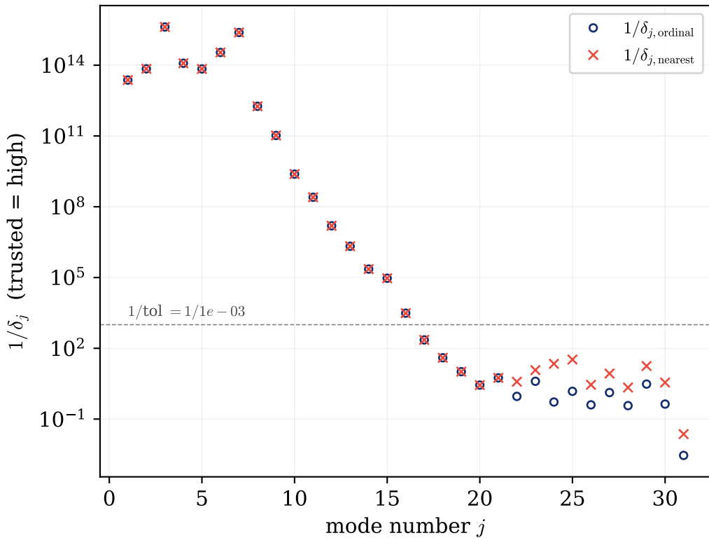
Dirichlet Laplacian, N_1 = 32, N_2 = 48
