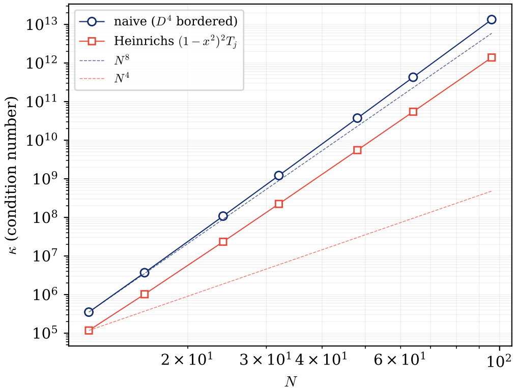
conditioning of the fourth-derivative matrix
