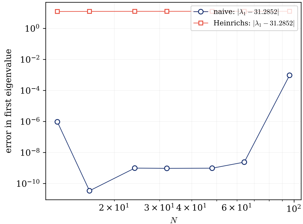
first-eigenvalue error vs. N
