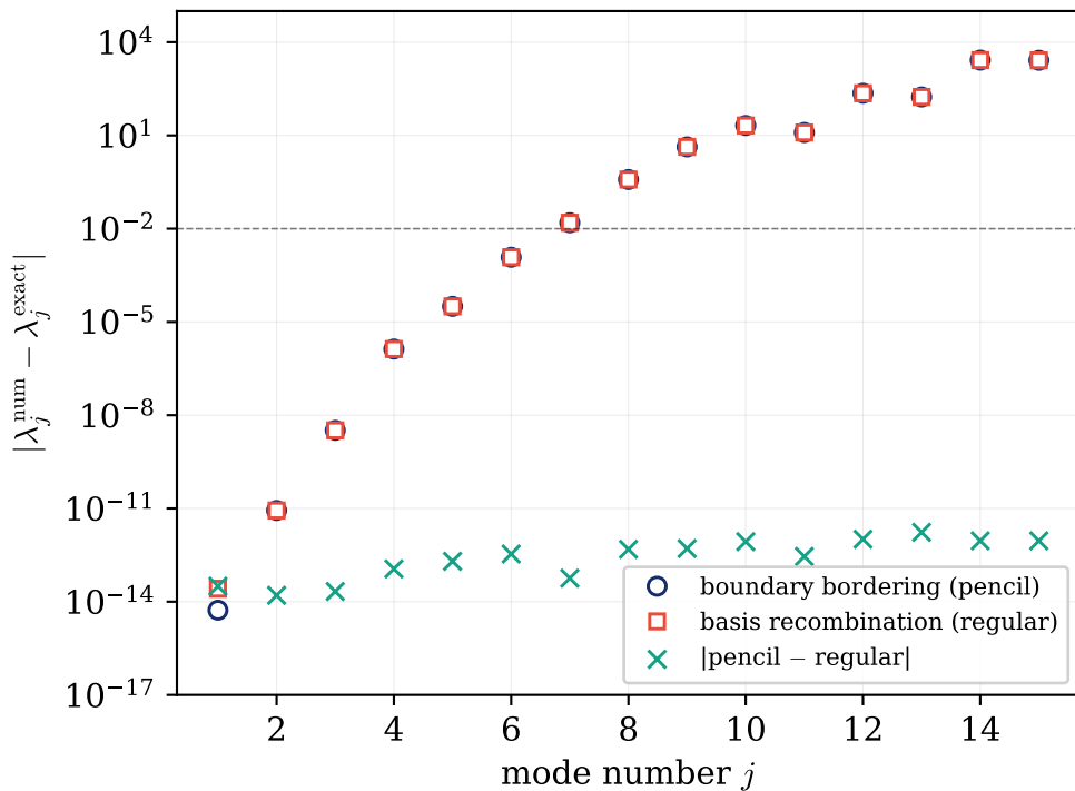
both formulations, N = 16
