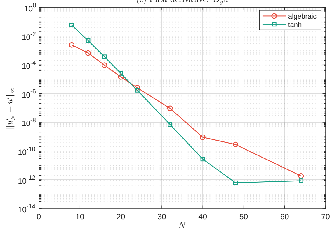
(c) First derivative: D_y u
