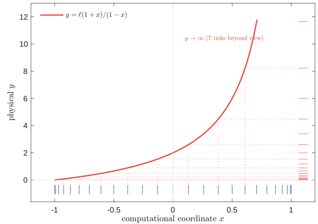
(b) algebraic map ( \ell = 2 ): clusters near y = 0
