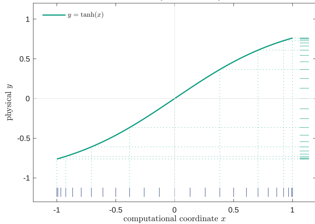
(a) tanh map: x_j (bottom) \rightarrow y_j (right)
