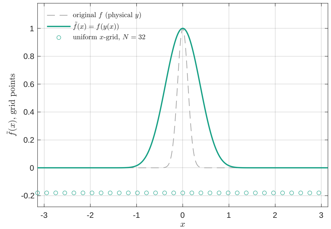
(b) Pulse in computational x
