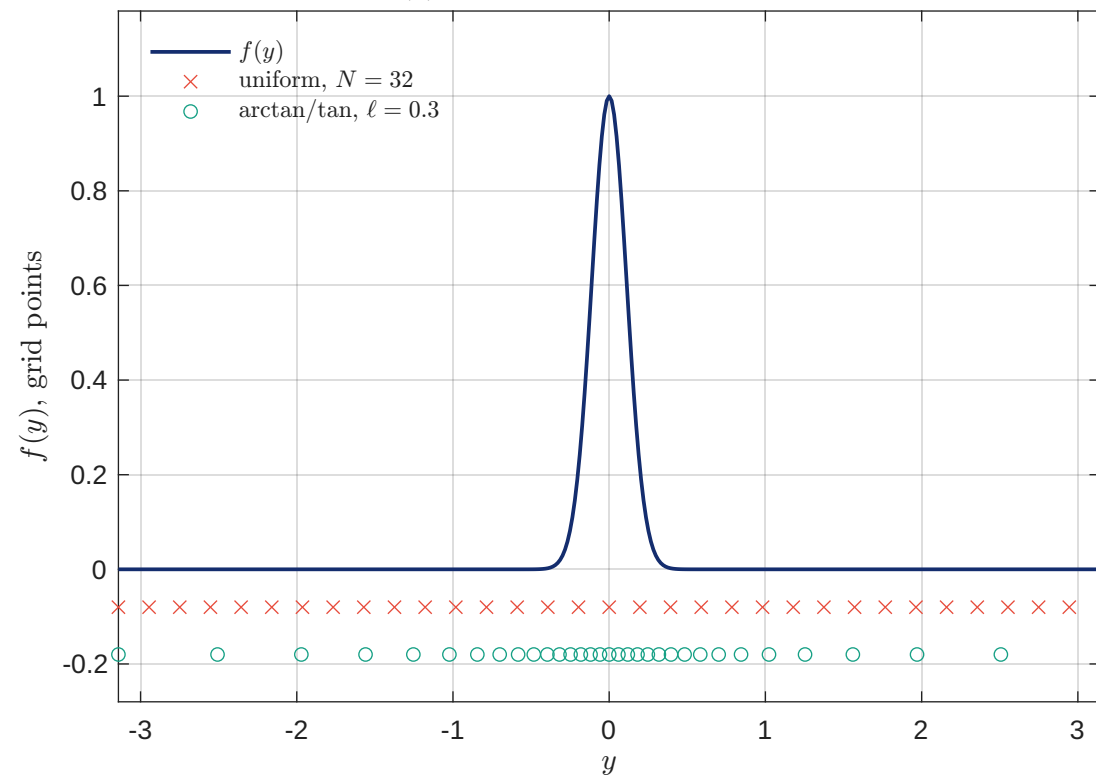
(a) Pulse and grids in physical y
